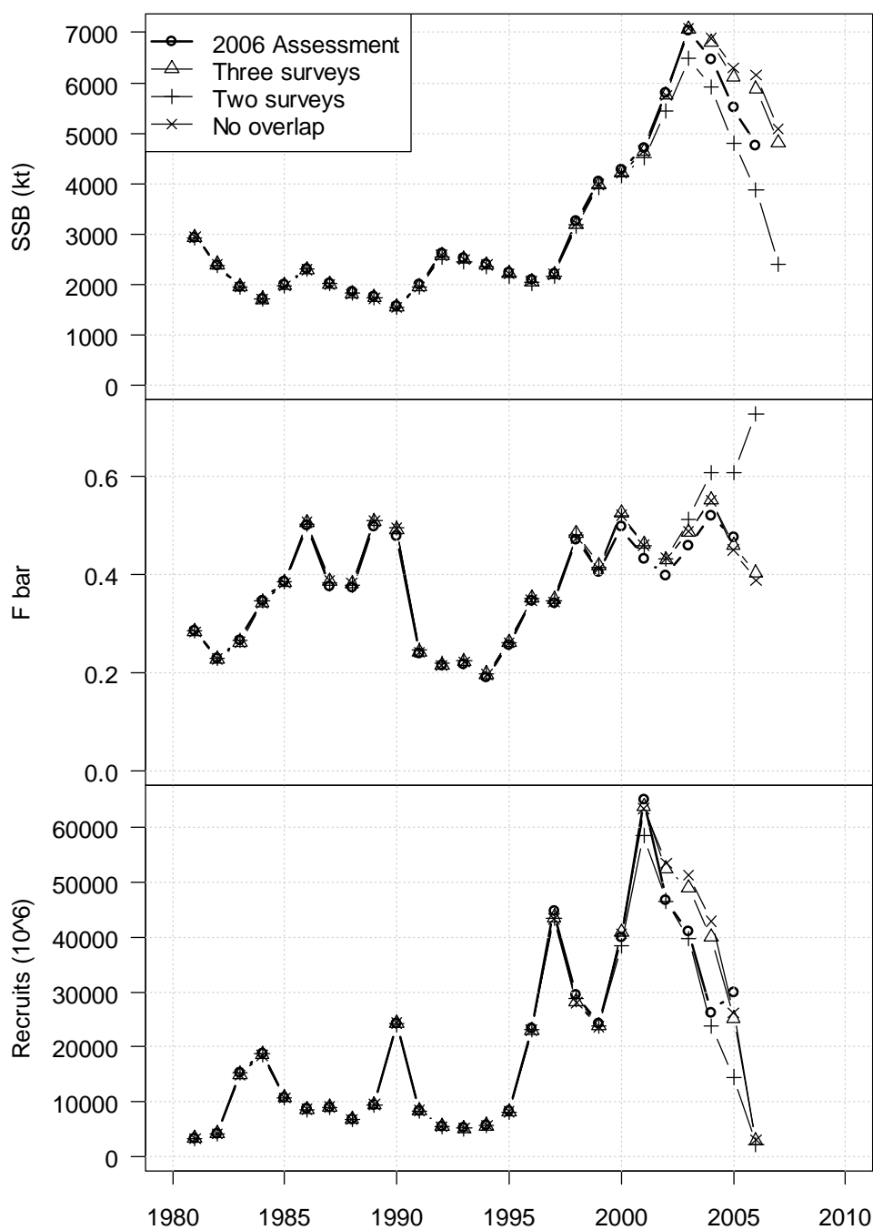
Figure 4.3.6.1. Blue Whiting SMS exploratory runs. Results of the three exploratory runs showing SSB (top panel), mean fishing mortality, \bar{F} bar (ages 3–7; middle panel) and estimated recruitment (bottom panel). For comparison, the results of the blue whiting assessment made with SMS during the 2006 WGNPBW are shown. The “two surveys” run can be considered as an ASPALY (Almost the Same Procedure as Last Year) run.
