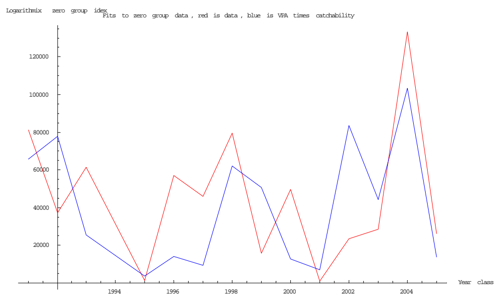
Figure 3.3.3.11. Norwegian spring spawning herring. Expectation values from the VPA (blue line) and zero group observations (red line) as estimated by SeaStar.
