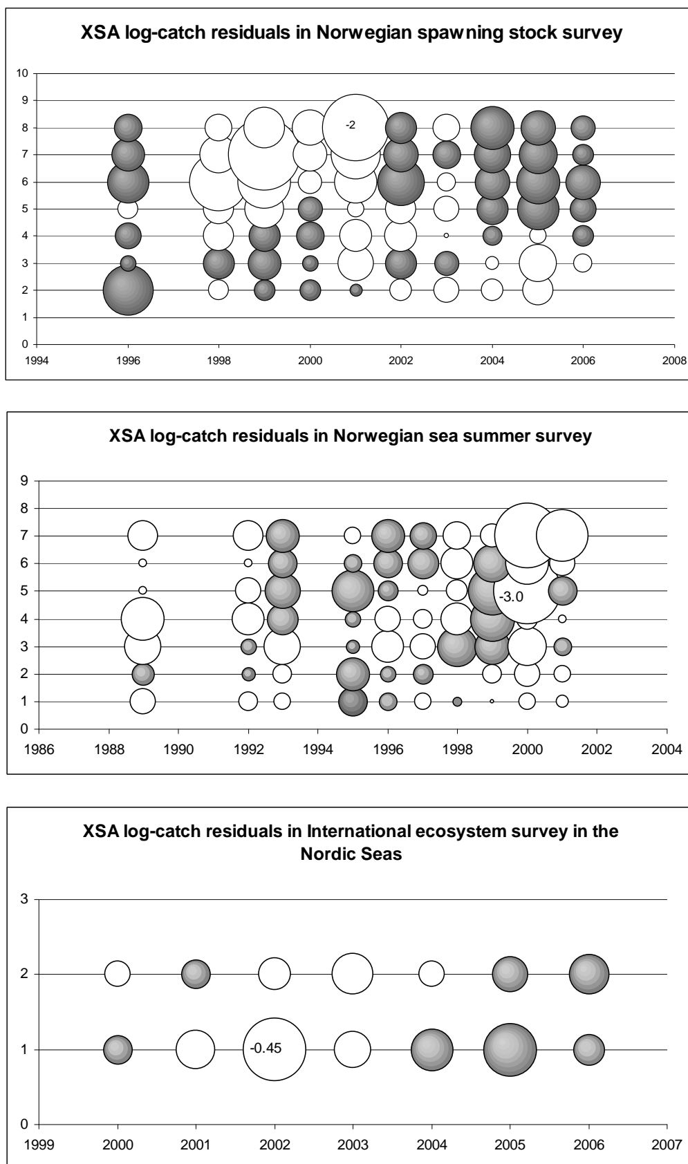
Figure 4.3.7.2. Blue Whiting, XSA. Residual plots from final runs.
