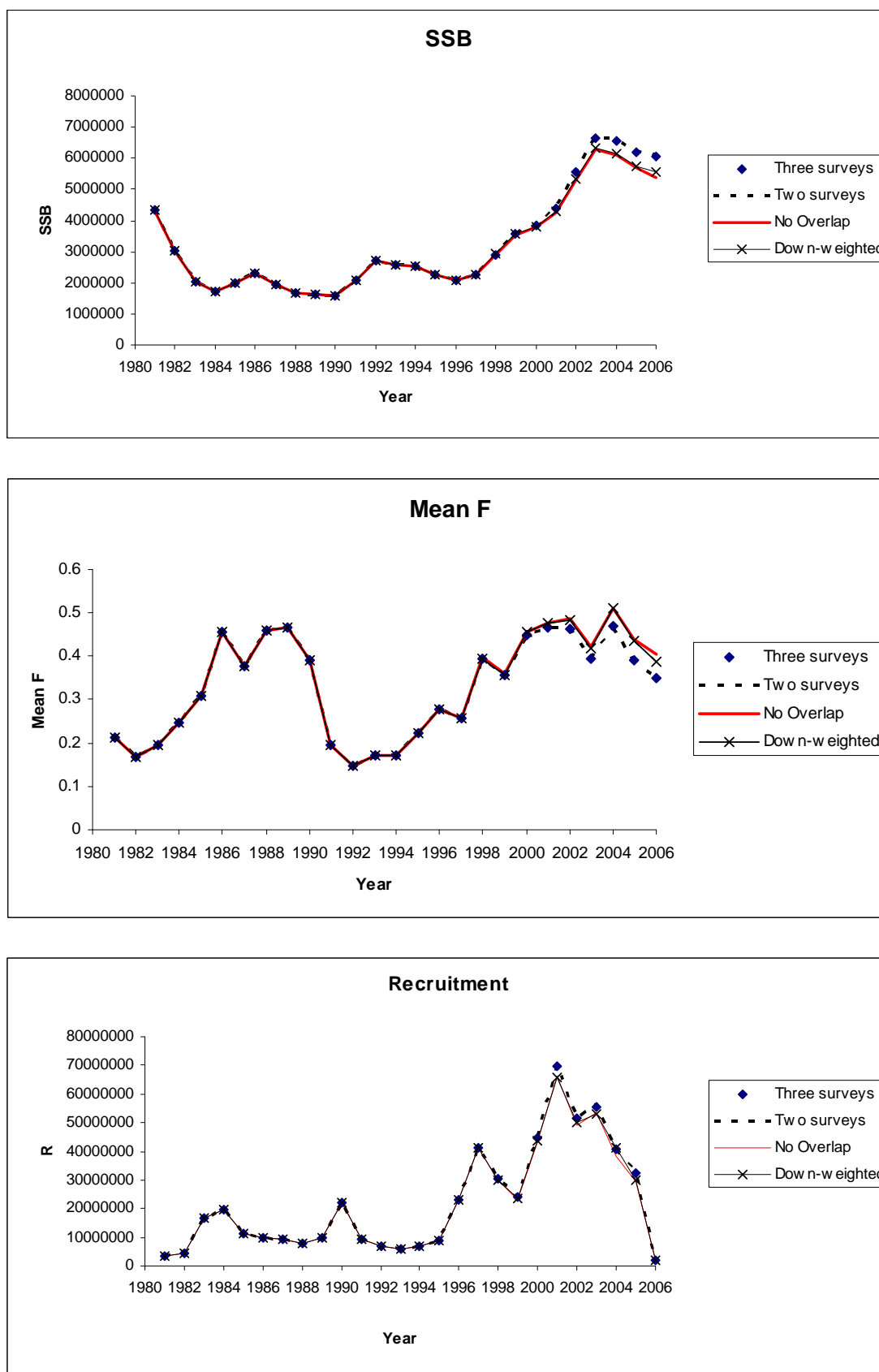
Figure 4.3.5.1. Blue Whiting. Comparisons of the ICA runs.
