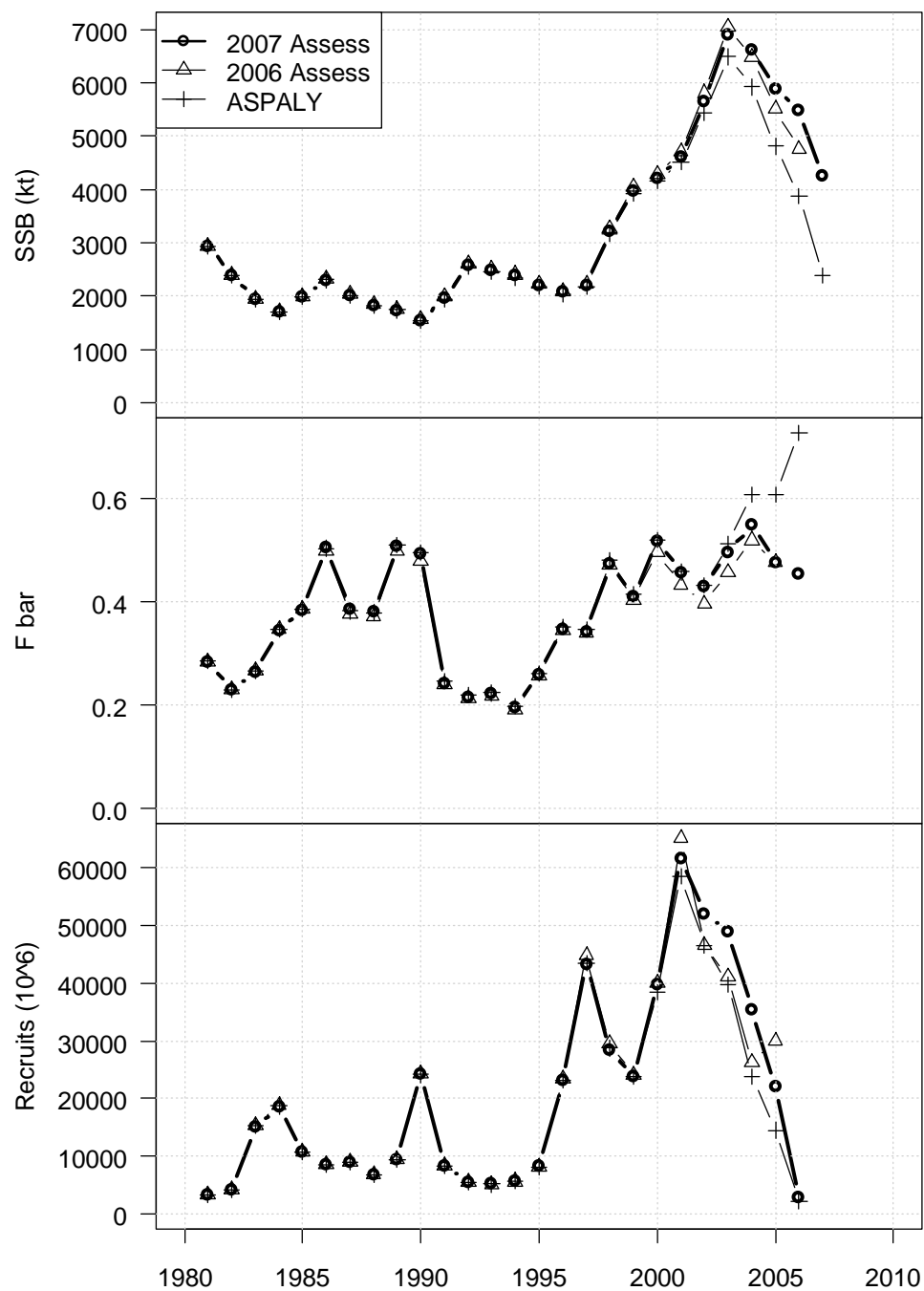
Figure 4.3.6.7. Blue whiting SMS data exploration. Quality plot for final SMS run. Time series of estimated SSB (top panel), mean fishing mortality, F_{bar} (ages 3–7; middle panel) and estimated recruitment (bottom panel) from the SMS method. For comparison, the results of the blue whiting assessment made with SMS during the 2006 WGNPBW, and the “Almost Same Procedure as Last Year” (ASAPLY) run are shown. The ASPALY run uses the same configuration as the 2006 working group, with the inclusion of 2006 data; however, the absence of a 2007 Norwegian survey meant that it was not possible to fully replicate the previous years methodology, hence the “ASPALY” name.
