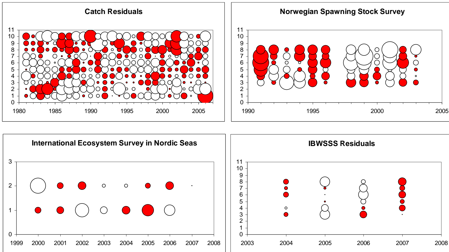
Figure 4.3.3.2. Blue whiting. AMCI final run. Catch and Survey Residual Patterns.
