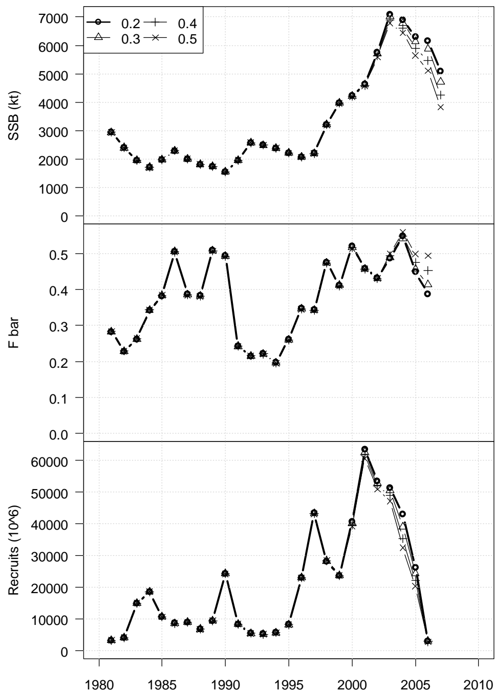
Figure 4.3.6.3. Blue Whiting SMS data exploration. Effect on SSB (top panel), mean fishing mortality, F_{bar} (ages 3–7; middle panel) and estimated recruitment (bottom panel) of the “minimum CV [standard deviation in log-normal distribution] on survey observations” constraint. Values less than 0.2 gave results indistinguishable from the 0.2 line. The minimum standard deviation of the survey observations was set to be 0.2 to 0.5 and the a priori weighting on the catches and surveys were both set to be 1.
