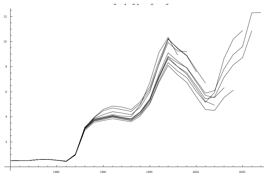
Figure 3.4.2.1. Norwegian spring spawning herring. Retrospective analysis for the SeaStar assessment. The same settings and the same algorithm for selecting year classes to be estimated in stage 1 and 2 are applied for each starting year. See text for details. Years are on x-axis and ssb on y-axis in million tonnes.
