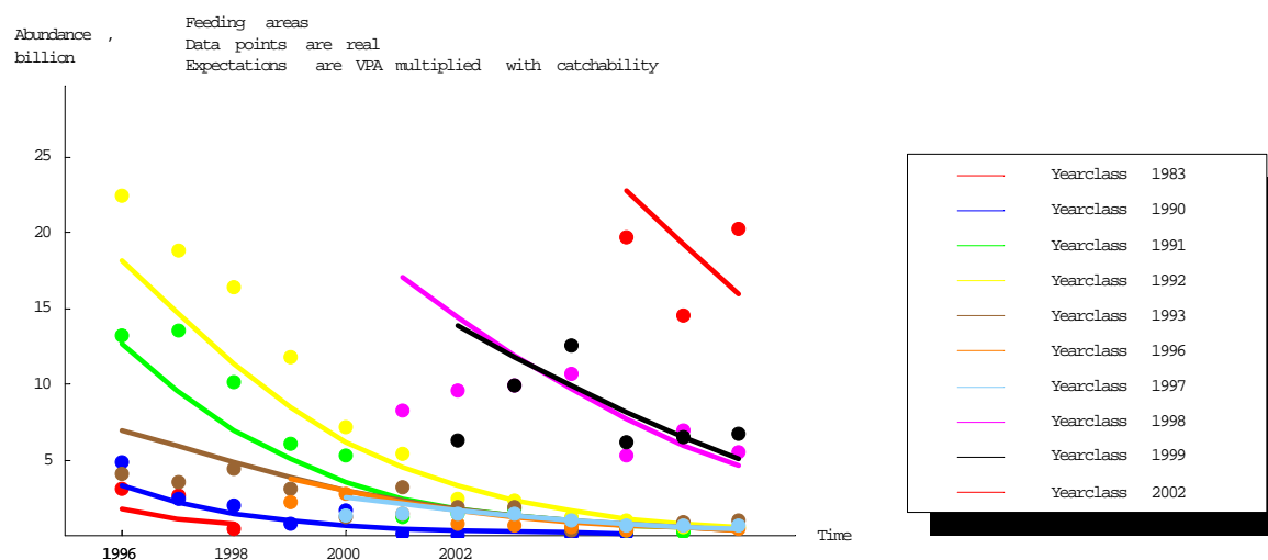
Figure 3.3.3.7. Norwegian spring spawning herring. Expectation values from the VPA (solid lines) and survey observations (dots) for survey 5 (feeding grounds in the Norwegian Sea in May-June) as estimated by SeaStar.
