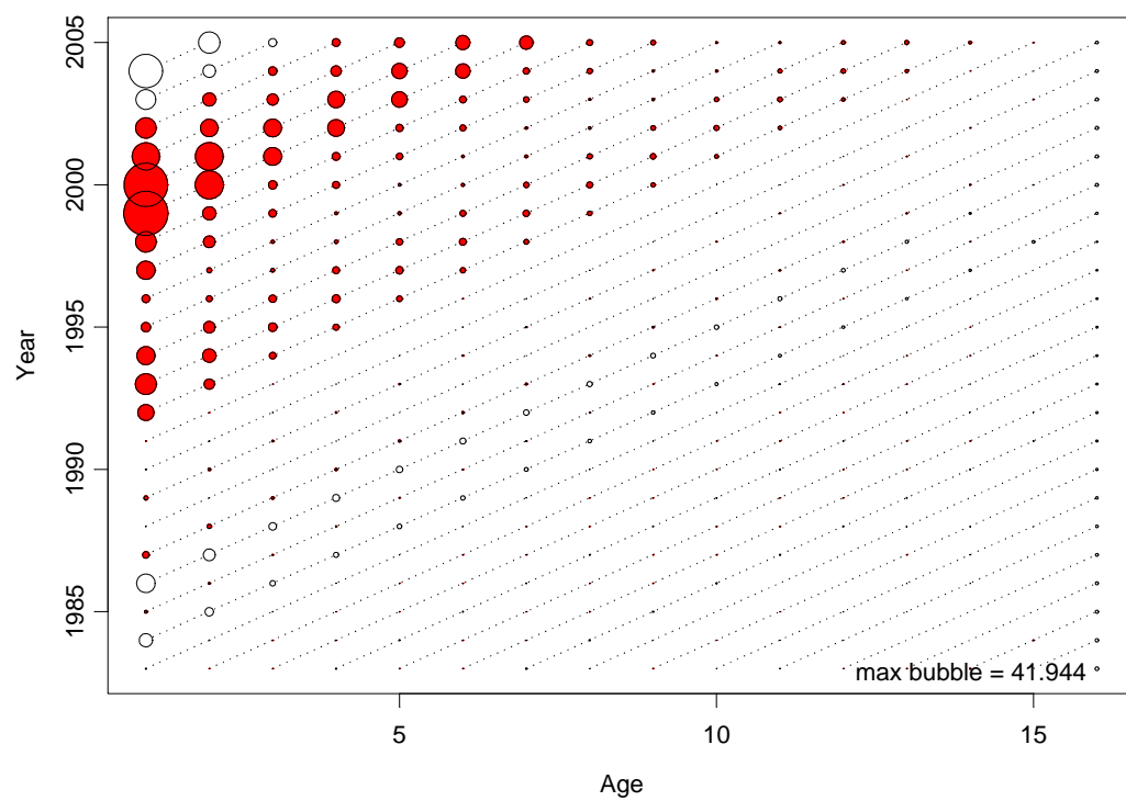
Figure 3.7.3.1 Difference of stocknumbers using surveys 2 and 5: ISVPA-SeaStar.
