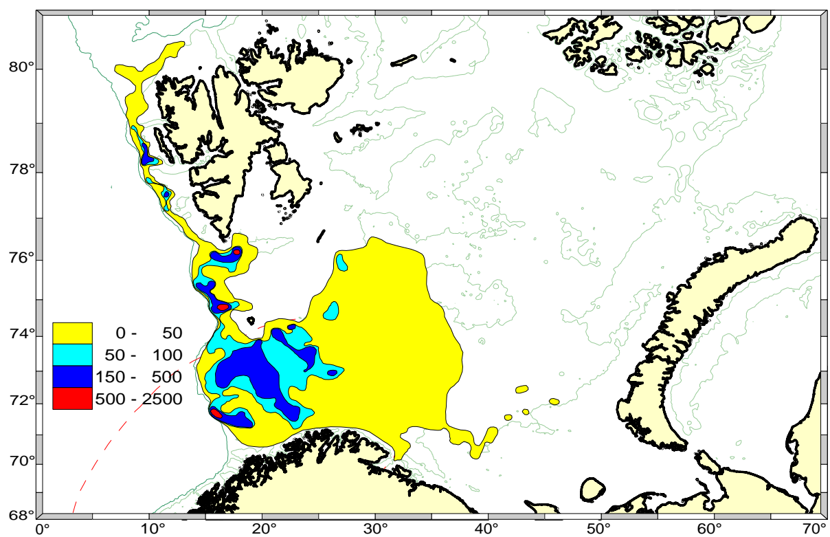
Fig. 4.6.1.8.1 Blue whiting distribution in October-December 2004 ( s_A , m^2/mile^2 ).
