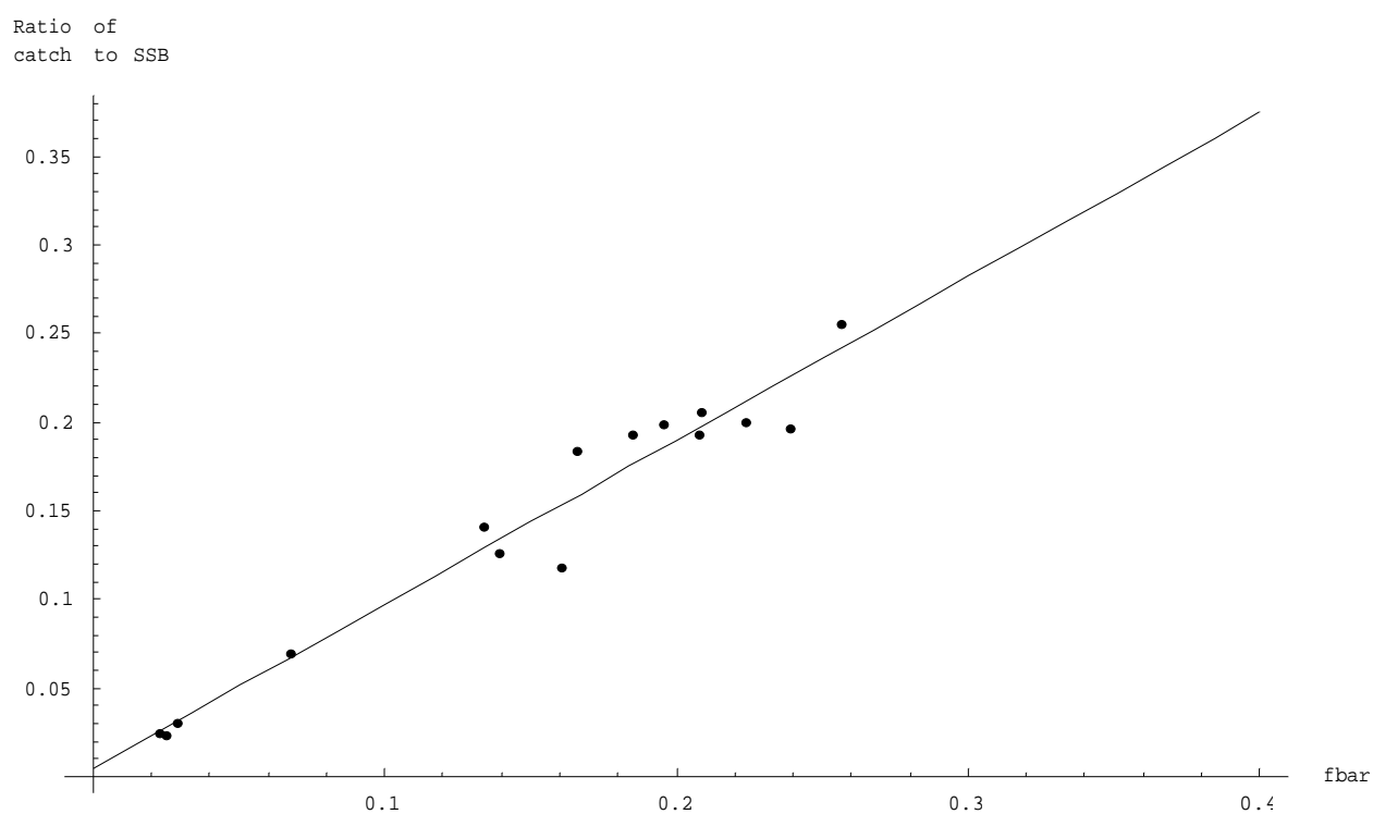
Figure 3.9.1.1 Ratio of catch to SSB regressed to Fbar. The fitted line has an intercept of 0.005 and a steepness of 0.93.
