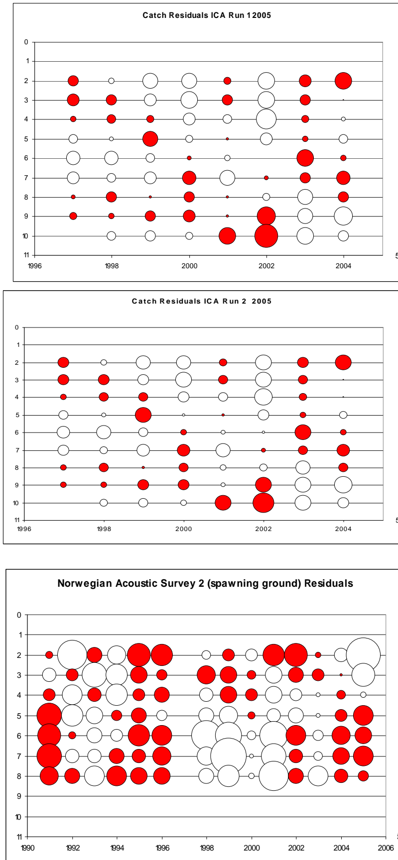
Figure 4.7.4.3. Residual plots for catches and survey for blue whiting, final run 2 WG 2005.
