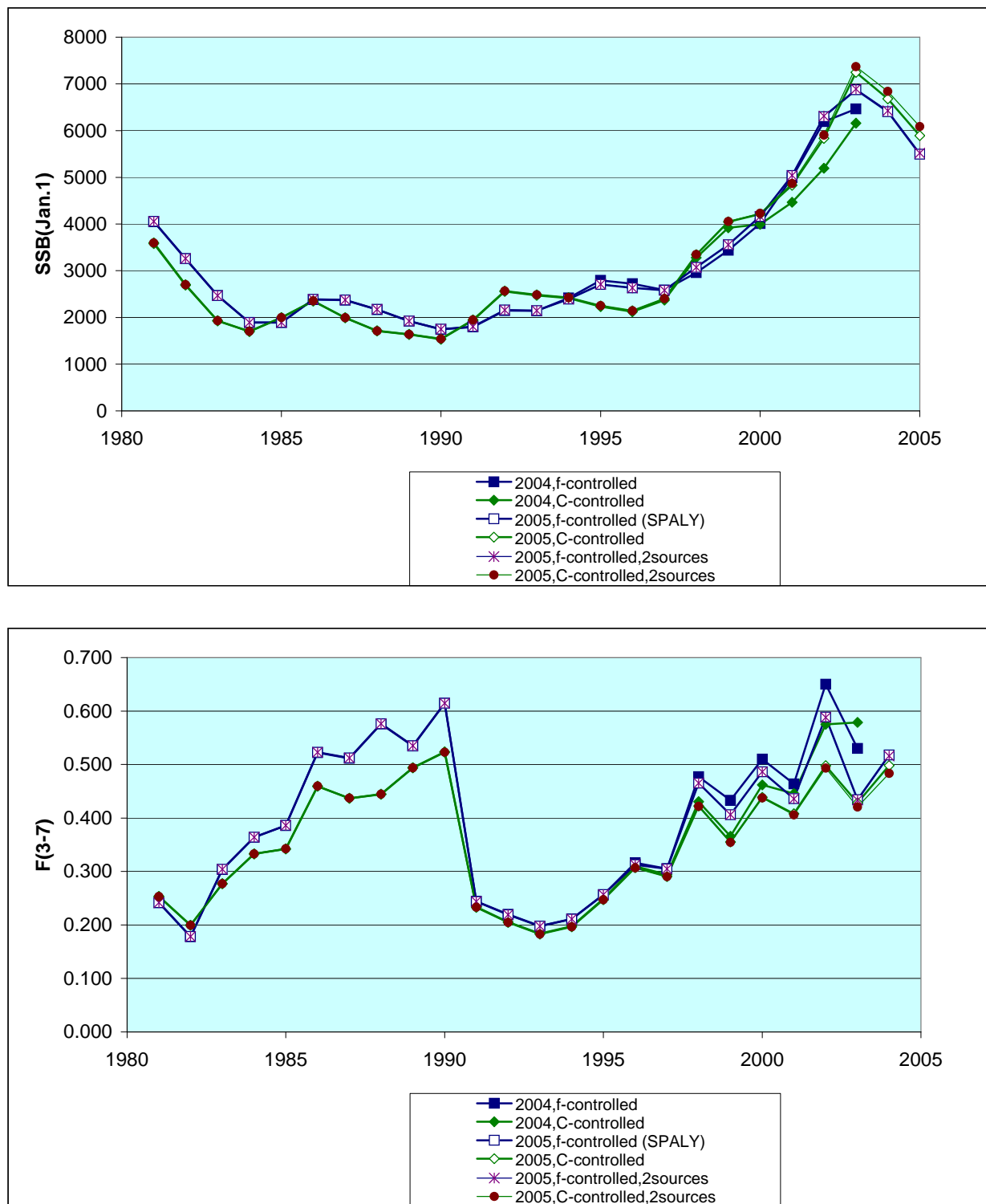
Figure 4.7.3.3 Blue whiting. Comparison of ISVPA-derived estimates in 2004 and 2005 assessments.
