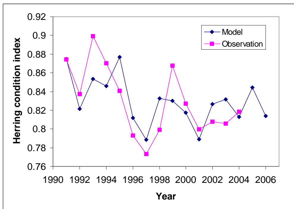
Fig. 2.2.1.3 Herring condition index in December, observed and modelled. Model: \text{Condition (yr2)} = 0.022 \cdot \text{NAO yr1} + 0.82 , R^2 = 0.51 , P = 0.004 . The model predicts herring condition index in December 2005 at 0.844 and in December 2006 at 0.82.
