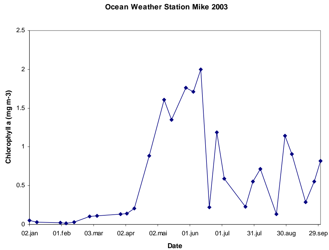
Figure 2.1.2.2.1 Distribution of chlorophyll a at 10 m depth during the year at Weather Station Mike in 2003.
