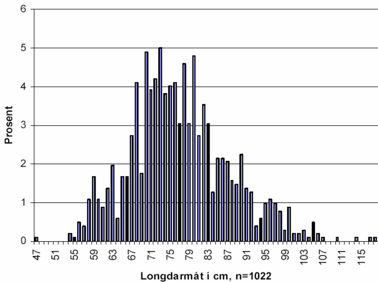
Figure 4.4.2.2. Length distribution (percentage) in cm of by-catch of saithe caught in the screenings on board the factory trawler M/T Næraberg in November-December 2004 (Lamhauge 2004).
