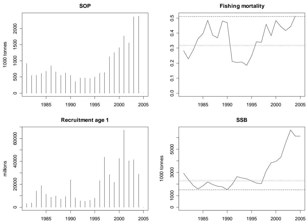
Figure 4.7.5.8 Blue Whiting, SMS. Stock summary, 1981-2005. For the calculation of SSB in 2005 an recruitment at 43.7 \times 10^9 is assumed.
