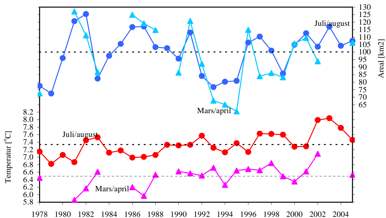
Figure 2.1.2.1.3. Time series of area (blue, in km 2 ) and averaged temperature (red/pink) of Atlantic water in the Svinøy section, observed in March/April (triangles) and July/August (dots) 1978-2005.
