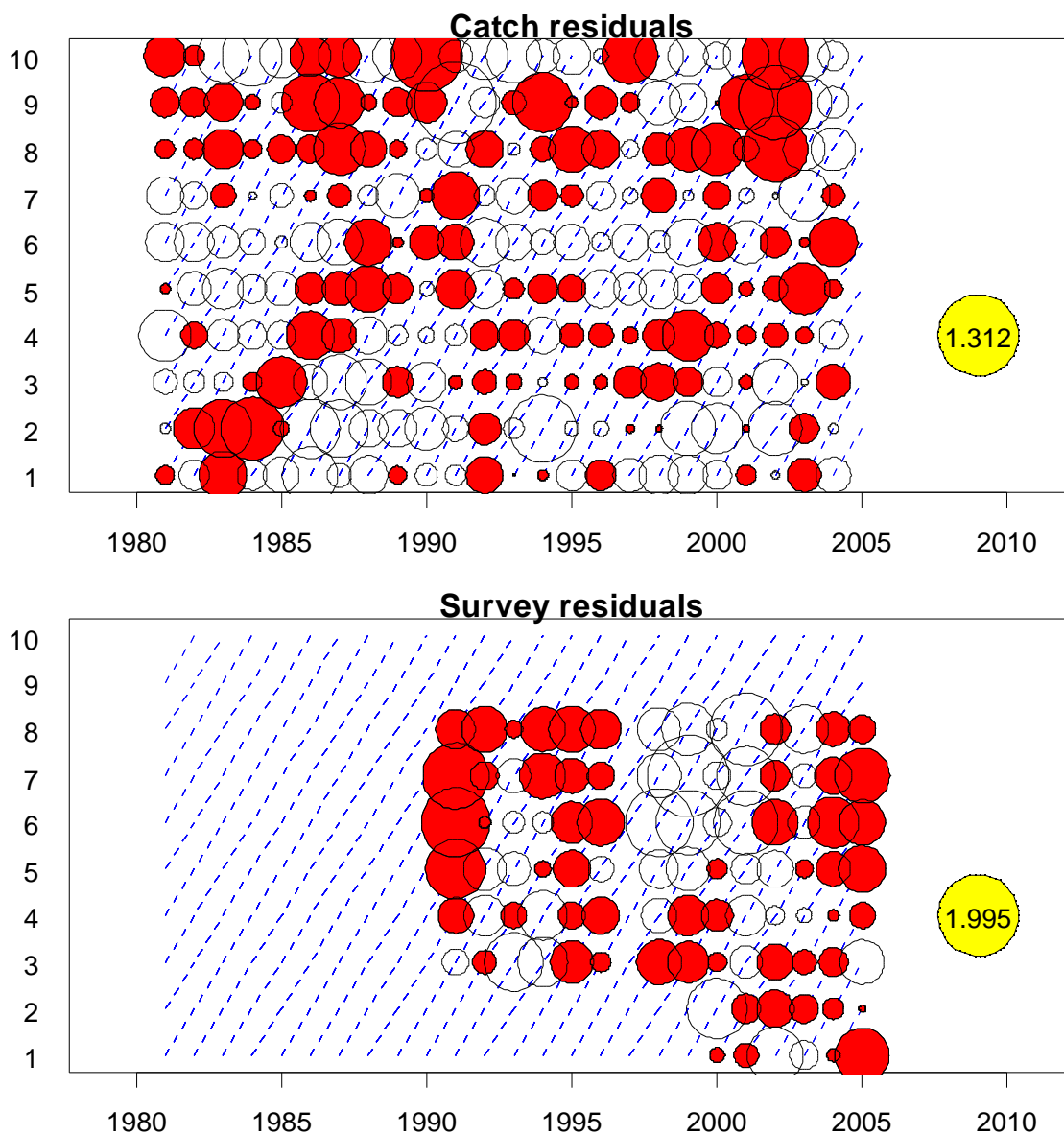
Figure 4.7.2.2. Blue whiting. Residuals from the final AMCI run. In the lower panel, residuals from two surveys are plotted in the same figure: Norwegian spawning stock survey (ages 3-8 years) and international May survey (ages 1-2 years).
