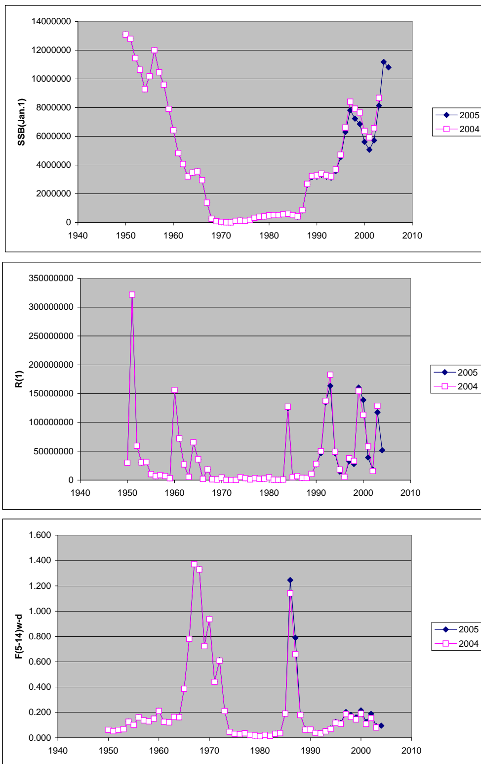
Figure. 3.7.2.2.5. NSS herring. ISVPA. Comparison to previous assessment
