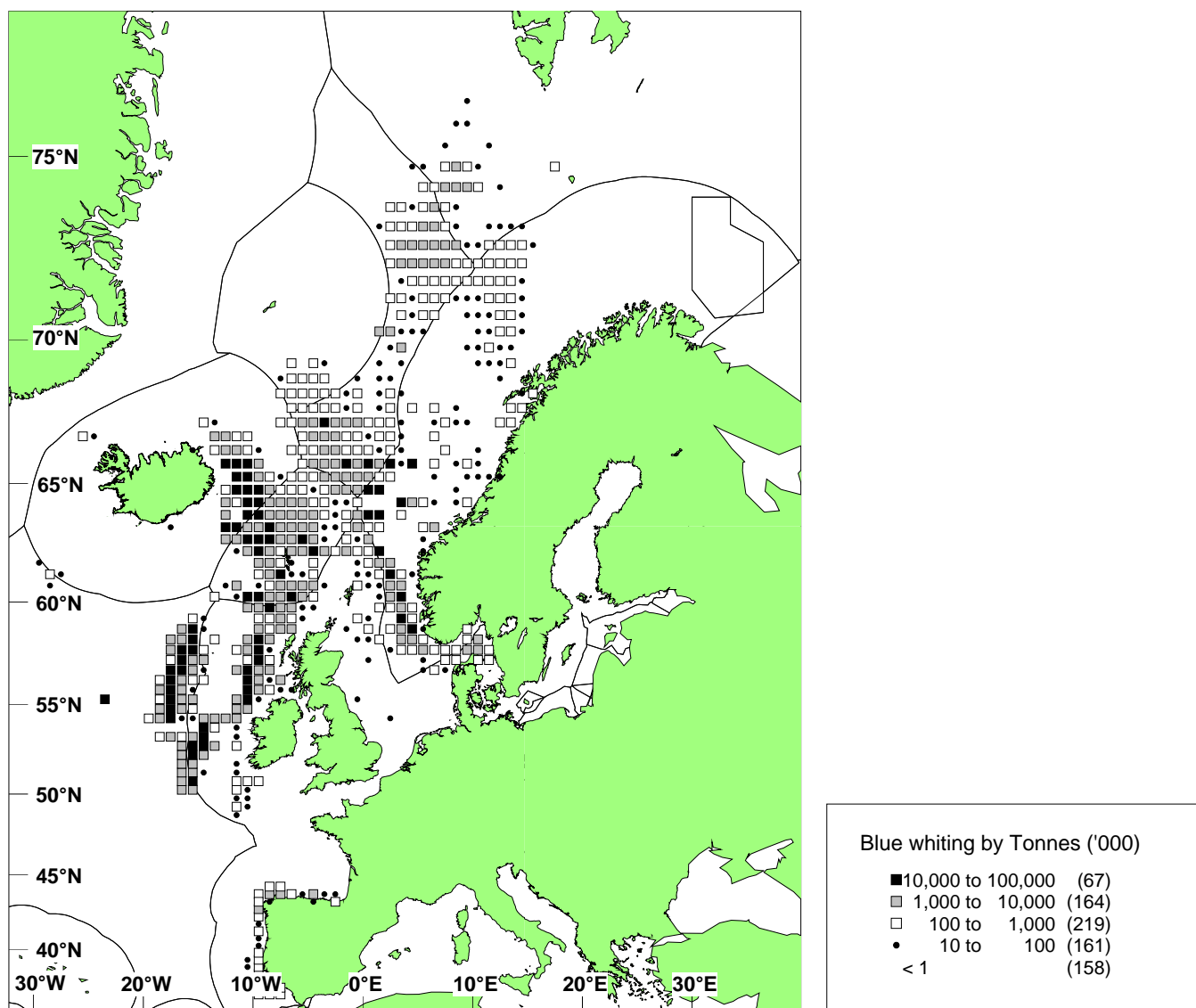
Figure 4.3.1. Total catches of blue whiting in 2004 by ICES rectangle. Grading of the symbols: small dots 10-100 t, white squares 100-1 000 t, grey squares 1 000-10 000 t, and black squares > 10 000 t.
