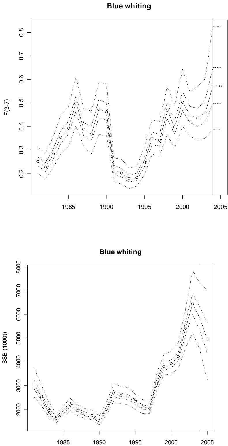
Figure 4.7.5.12 Blue Whiting, SMS. Posterior density (2.5, 25, 50, 75 and 97.5 percentiles) of average F and SSB estimated from 200000 Markov Chain Monte Carlo simulations. Recruitment in 2005 is assumed as the GM of the full time series.
