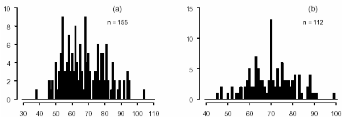
Fig. 4.4.1.3. Length distributions (numbers) of by-catch of (a) cod and (b) saithe in the Icelandic blue whiting fishery 2004 (Pálsson et al. 2004).
