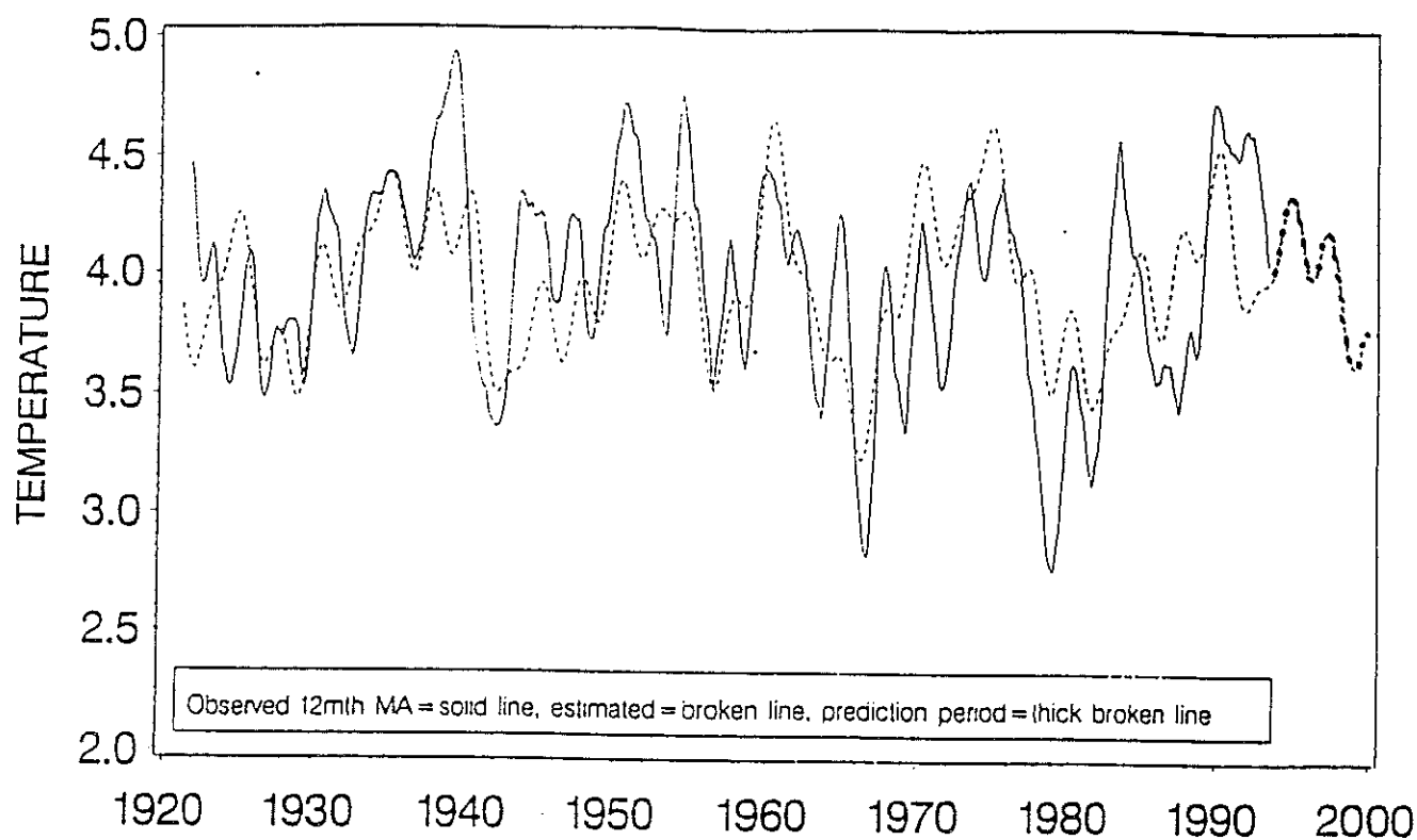
Figure 3.5 12 months moving average of monthly means of observed ocean temperature at the Kola section 1921-93, estimated values 1921-1993 and values forecasted for 1994-99
