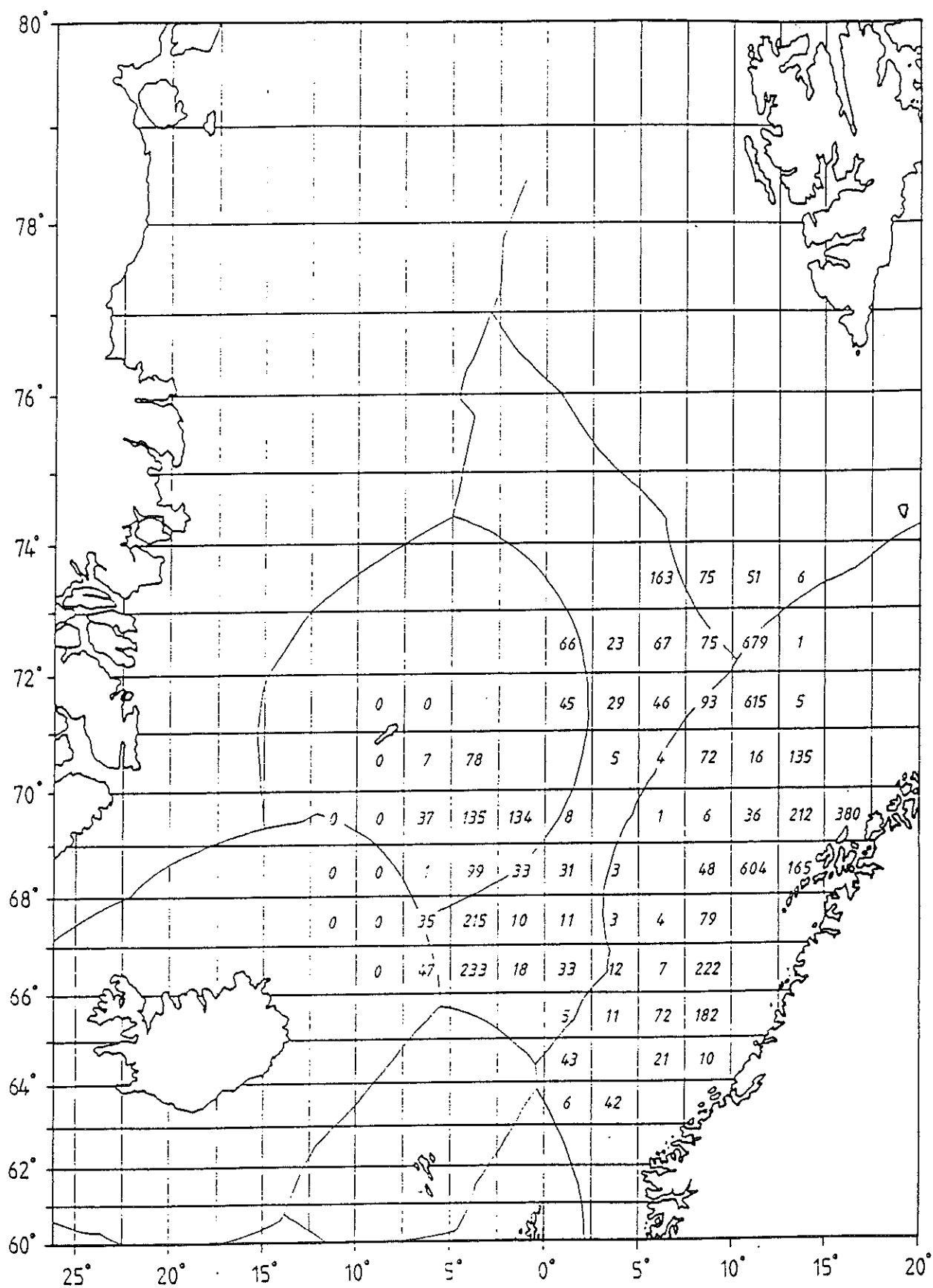
Figure 3.2 Norwegian spring spawning herring. Distribution of adult and adolescent herring in June - July 1994. Numbers denote average integrator values ( \text{m}^2/\text{n.m.}^2 .)
