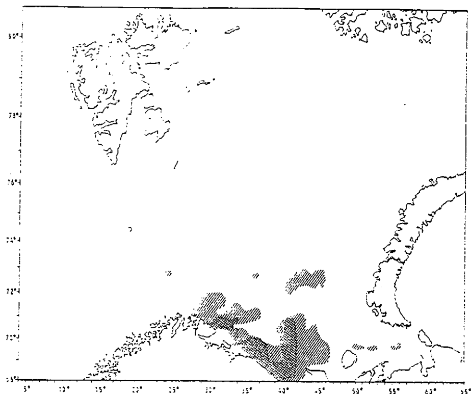
Figure 3.18 Norwegian spring spawning herring. A general picture of the distribution in 1994.
