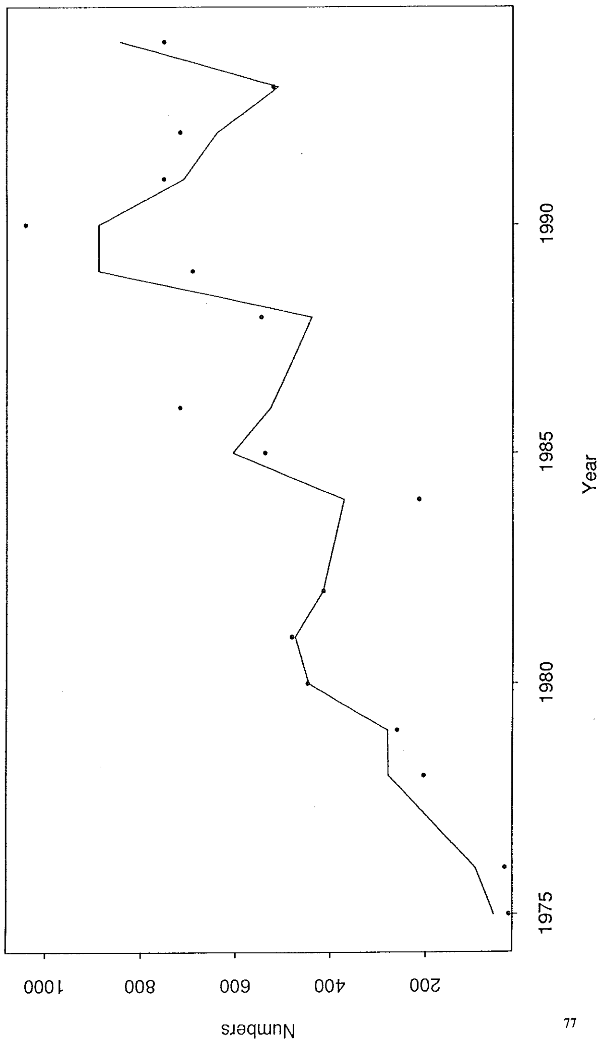
Figure 2. 4. Icelandic summer spawners. Trends in acoustics and VPA stock numbers.
