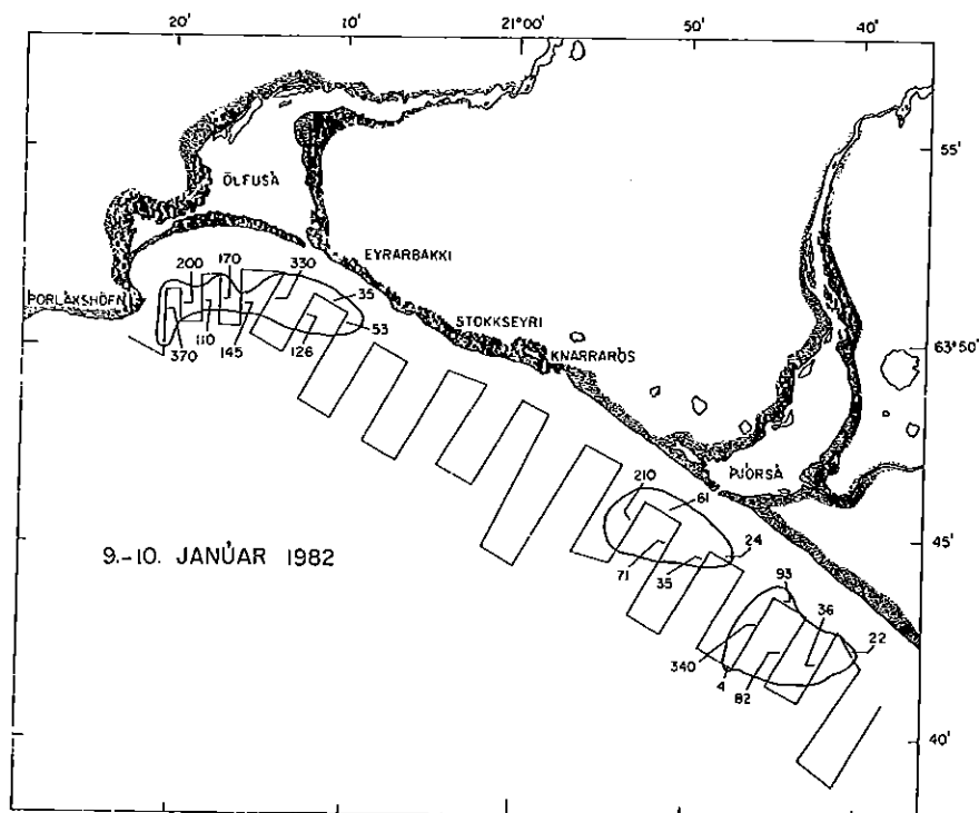
Figure 3. The winterring concentrations in January 1982. Echo intensities and distribution are shown on two successive nights.
