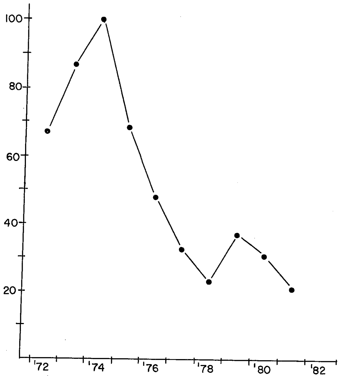
Figure 6. Relative abundance of 0-group capelin 1972-1981.
