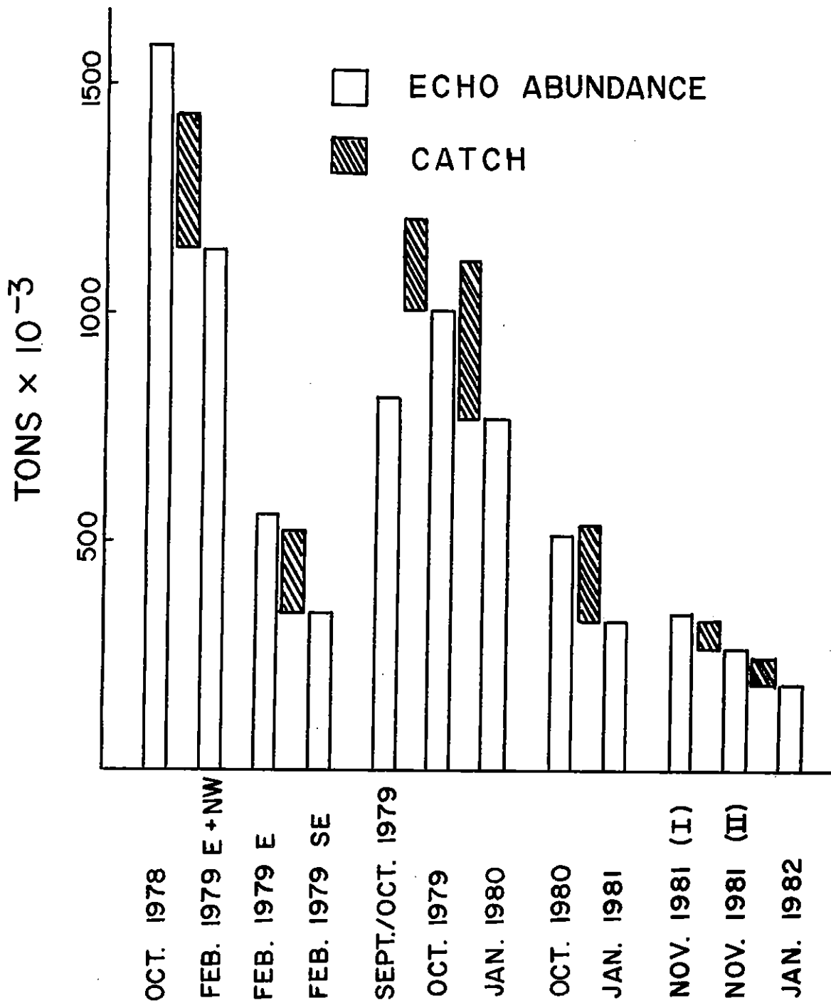
Figure 5. Successive acoustic abundance estimates of the Icelandic capelin stock and the catch during intervening periods, October 1978 - January 1982.
