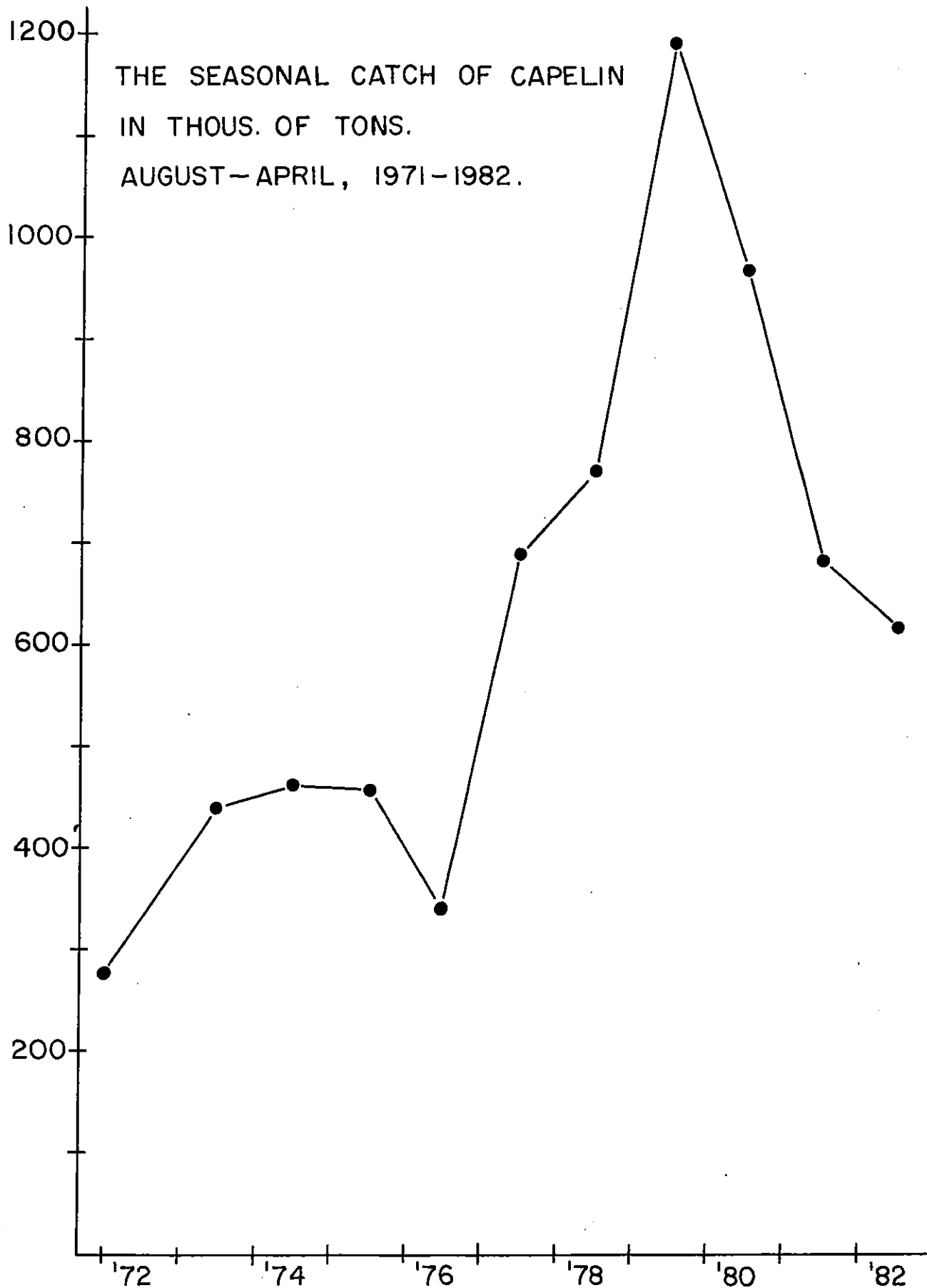
Figure 7. Seasonal catch of Capelin (in '000 tonnes) August-April, 1971-82.
