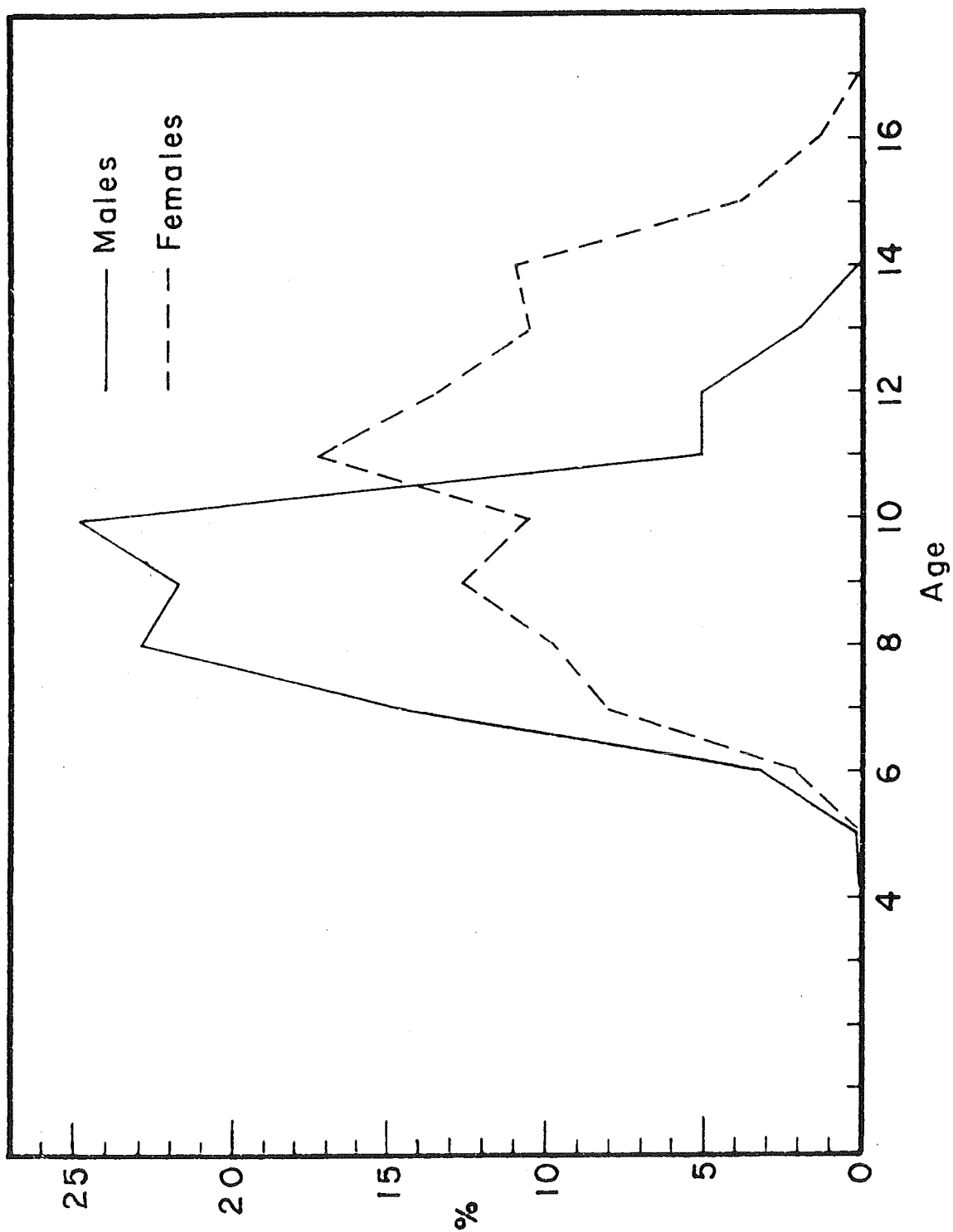
Appendix Figure 2. Greenland halibut in Division Va. The age distribution in the Icelandic long-line catches in 1976.
