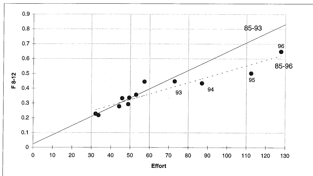
Figure 6.6.1. Plot of \bar{F} (8-12) versus total effort. \bar{F} values based on XSA with SE_{mshr} = 1.0 (Table 6.6.1.1) and effort based on Icelandic trawlfleet (Table 6.2.1). Linear relationships are shown for the two periods, 1985-93 and 1985-96.
