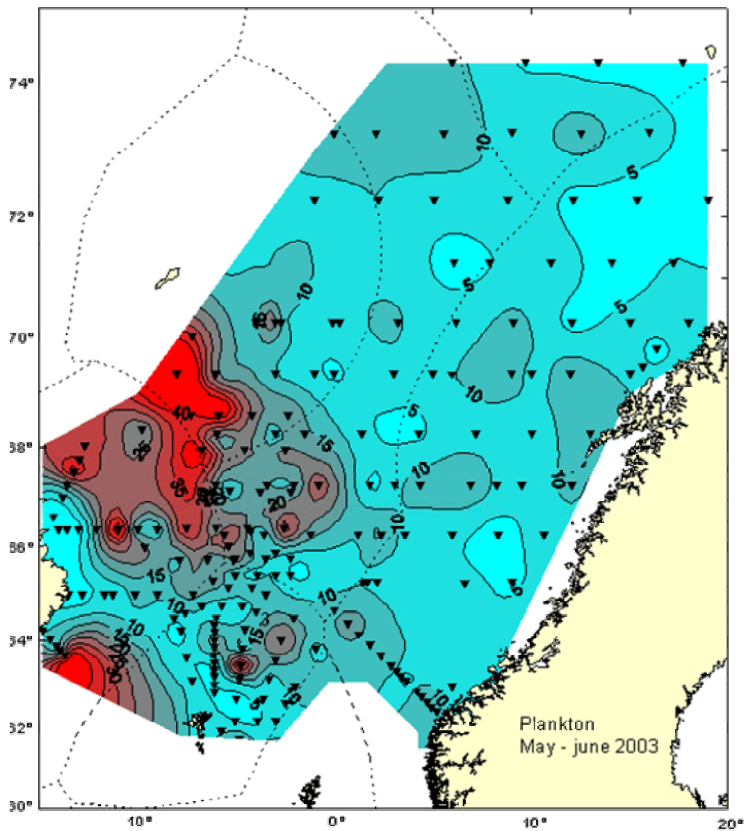
Figure 3.2.1 Zooplankton biomass ( \text{g dw m}^{-2} ) (200-0m) (50-0 m in Icelandic standard sections) in May 2003.
