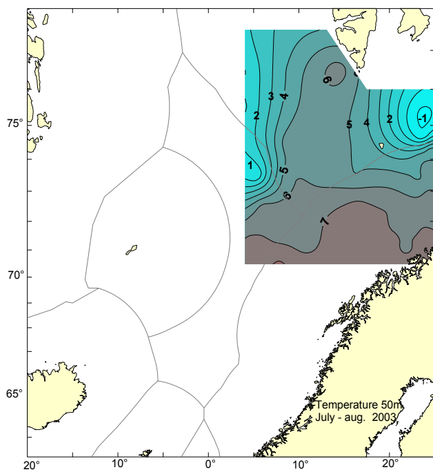
Figure 3.1.17 Temperature at 50 m depth in July/August 2003.
