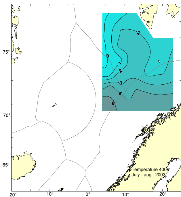
Figure 3.1.20 Temperature at 400 m depth in July/August 2003.
