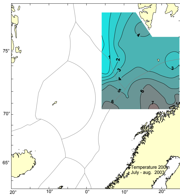
Figure 3.1.19 Temperature at 200 m depth in July/August 2003.
