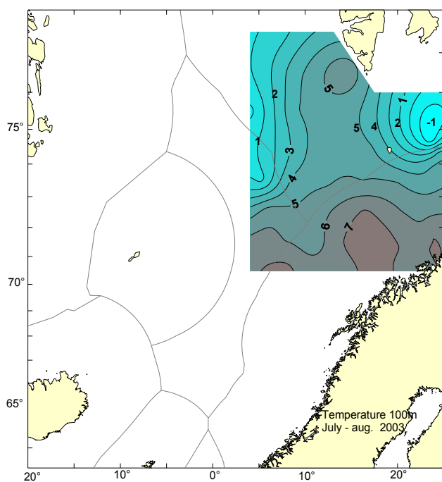
Figure 3.1.18 Temperature at 100 m depth in July/August 2003.
