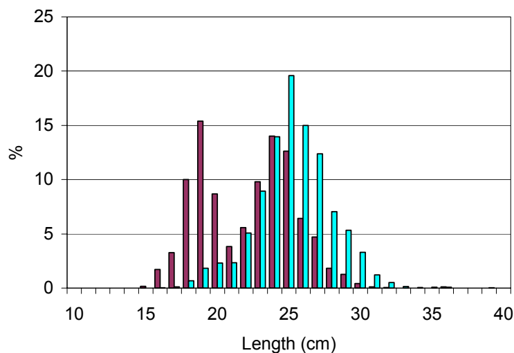
Figure 3.5.2 Length distribution of blue whiting in the southern part (< 62°N, dark bars) and in the northern part of the Faroese area sampled from R/V Magnus Heinason , May 2003.
