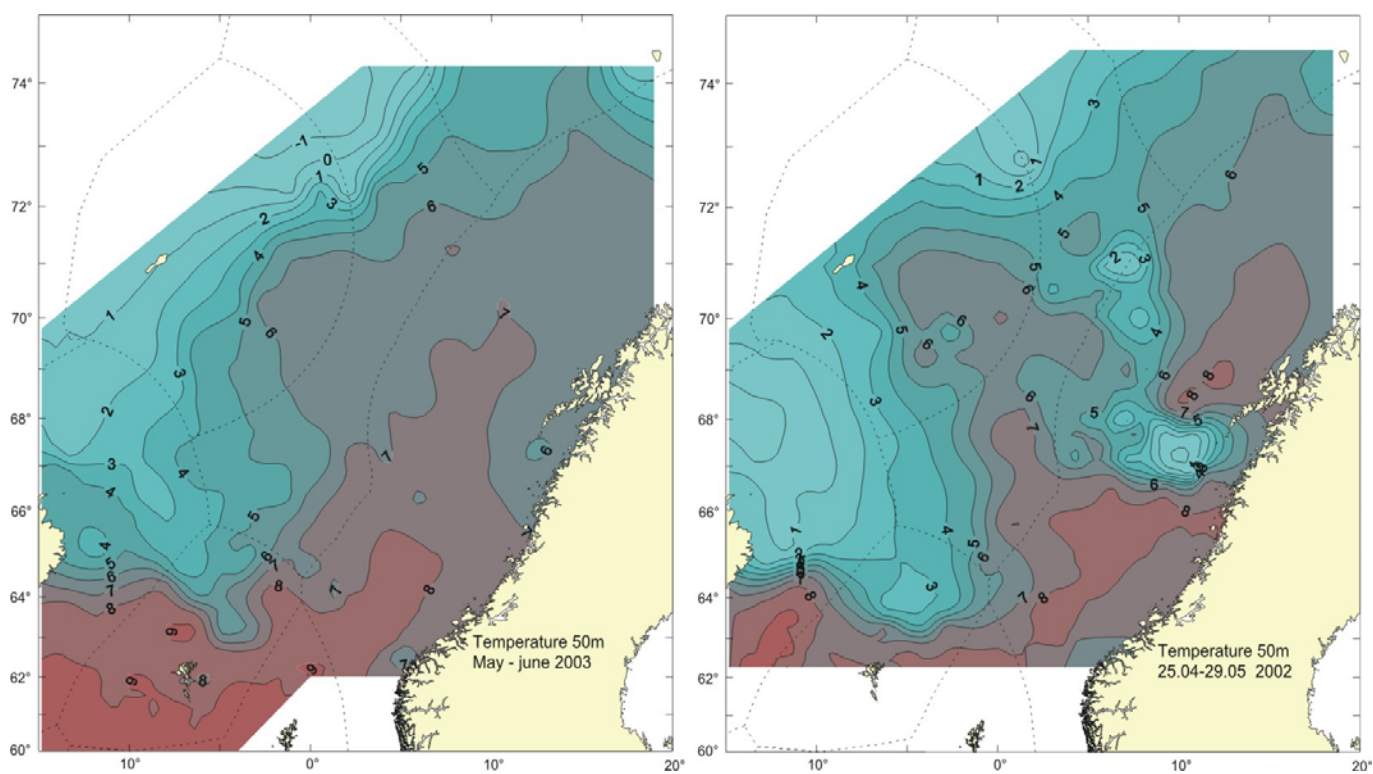
Figure 4.3.3 Temperature in 50 m in the Norwegian Sea in May 2003 (left) and 2002 (right).
