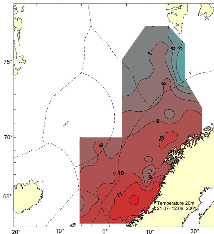
Figure 21. Temperatures at 20 meters in July-August 2001.
