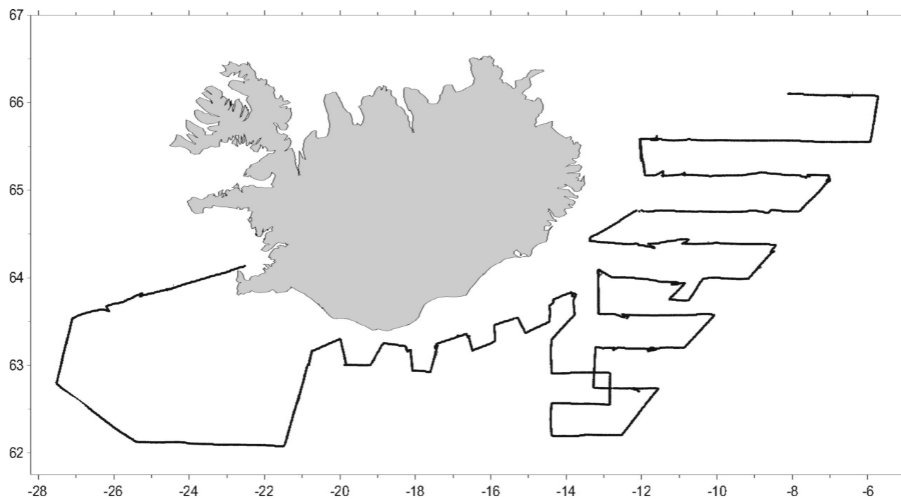
Figure 4. Survey tracks, R/V Arni Fridriksson, 17-30 July 2001.
