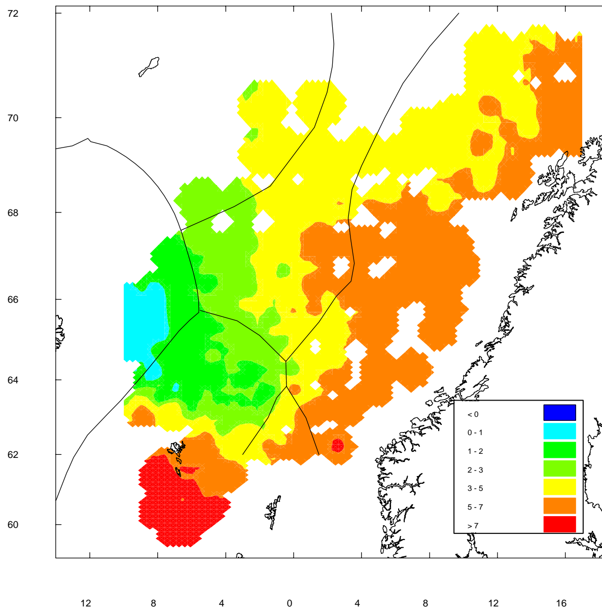
Figure 17. Temperature at 200 m in May 1997
