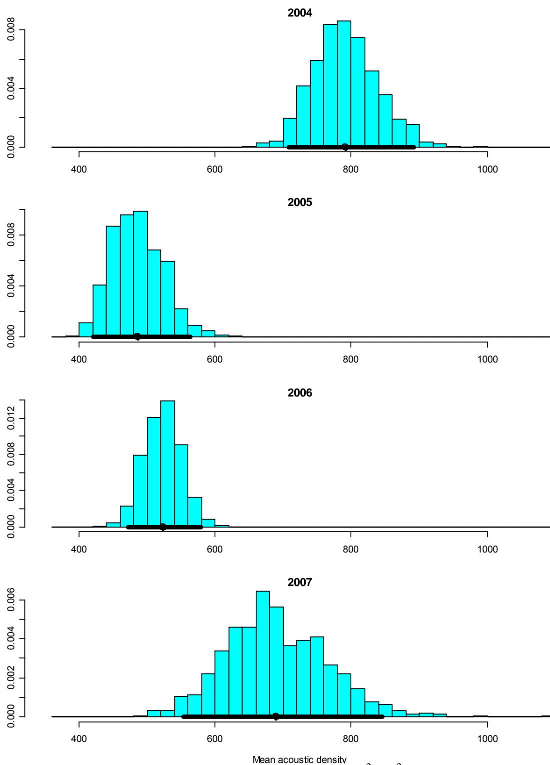
Figure 1. Distribution of mean acoustic density (in \text{m}^2/\text{nm}^2 ) based on 1000 bootstrap replicates of acoustic data from blue whiting surveys. Mean acoustic density is indicated with a black dot on the x-axis, while the horizontal bar shows 95% confidence limits.
