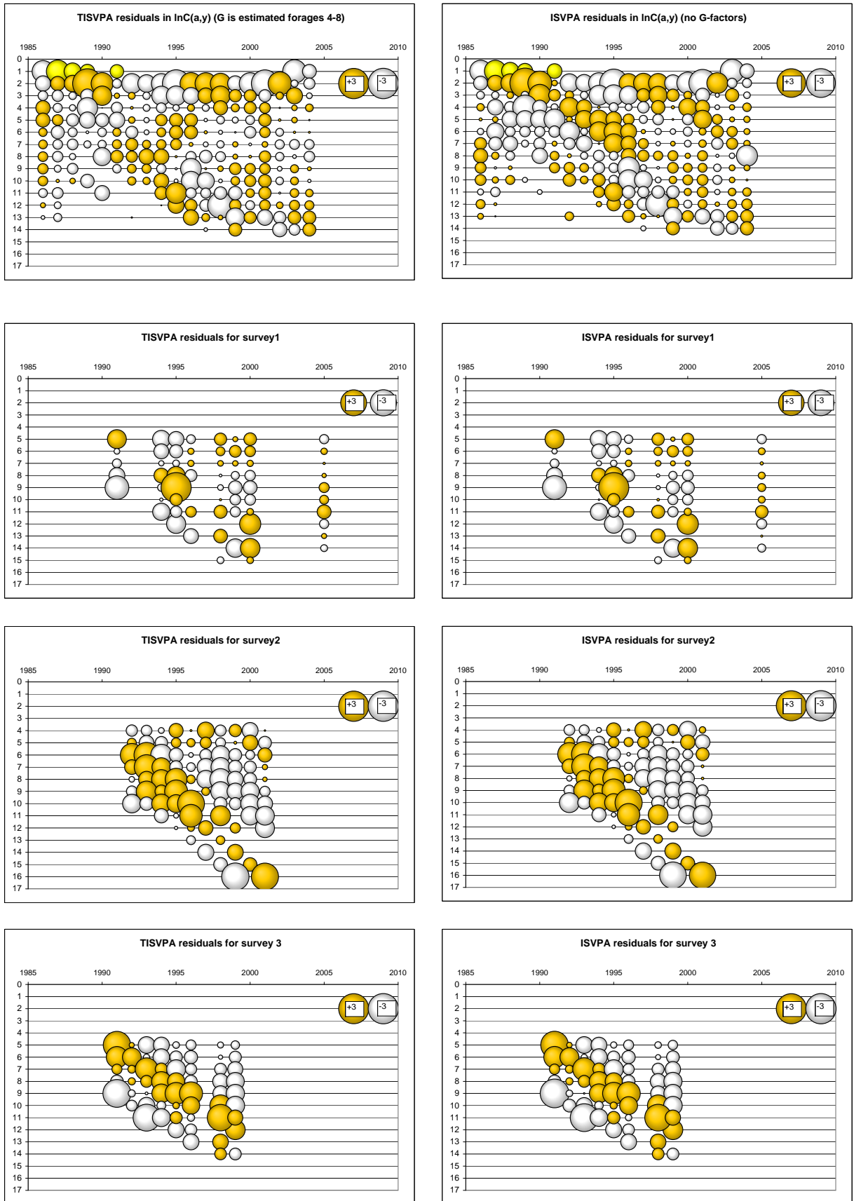
Figure 3.7.2.2.2 NSSH. Residuals in TISVPA and in ISVPA.
