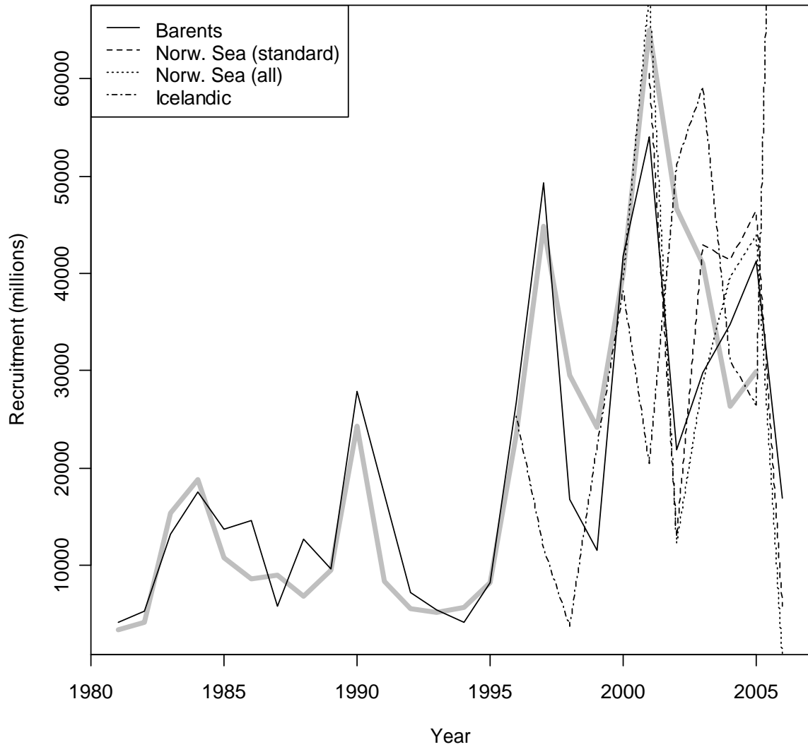
Figure 4.8.2. Blue whiting. Prediction of recruitment from survey data calibrated with the current stock assessment estimate (thick grey curve) for the period 1981–2004. Prediction based on the Barents Sea index is based on log-log regression. Other predictions are based on regressions forced through the origin in natural scale.
