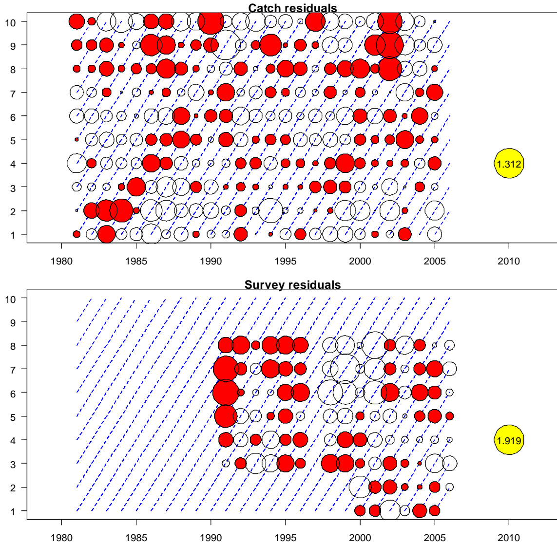
Figure 4.7.2.2. Blue whiting. Residuals from the final AMCI run. In the lower panel, residuals from two surveys are plotted in the same figure: Norwegian spawning stock survey (ages 3-8 years) and international Norwegian Sea ecosystem survey (ages 1-2 years).
