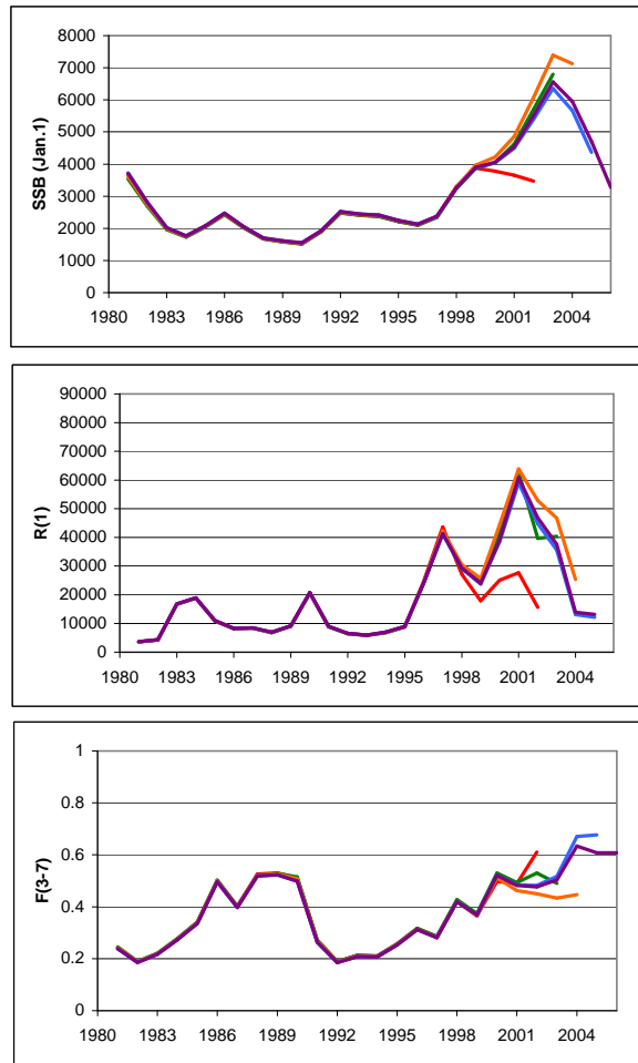
Figure 4.7.3.6 BW. TISVPA retrospective runs
