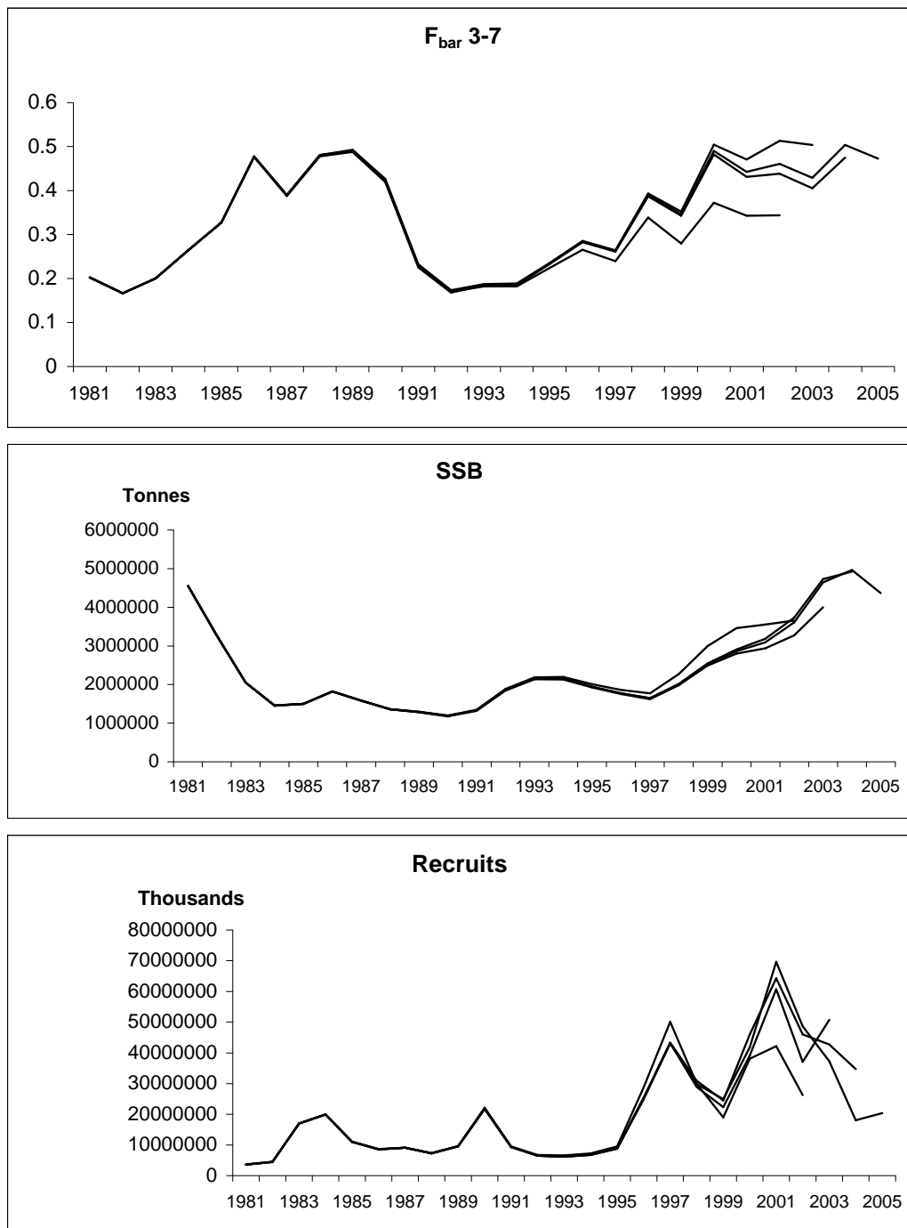
Figure 4.7.6.1. Blue Whiting. XSA results. Retrospective analysis.
