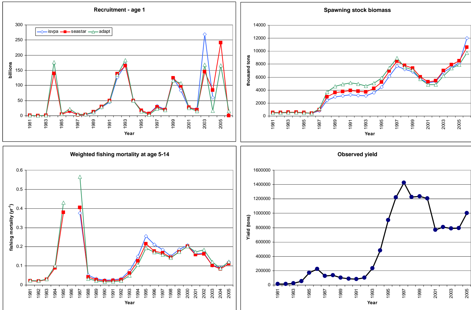
Figure 3.7.3.1 Norwegian spring spawning herring . Comparisons of results from assessments model ADAPT, ISVPA and SeaStar. (ISVPA from 1986).
