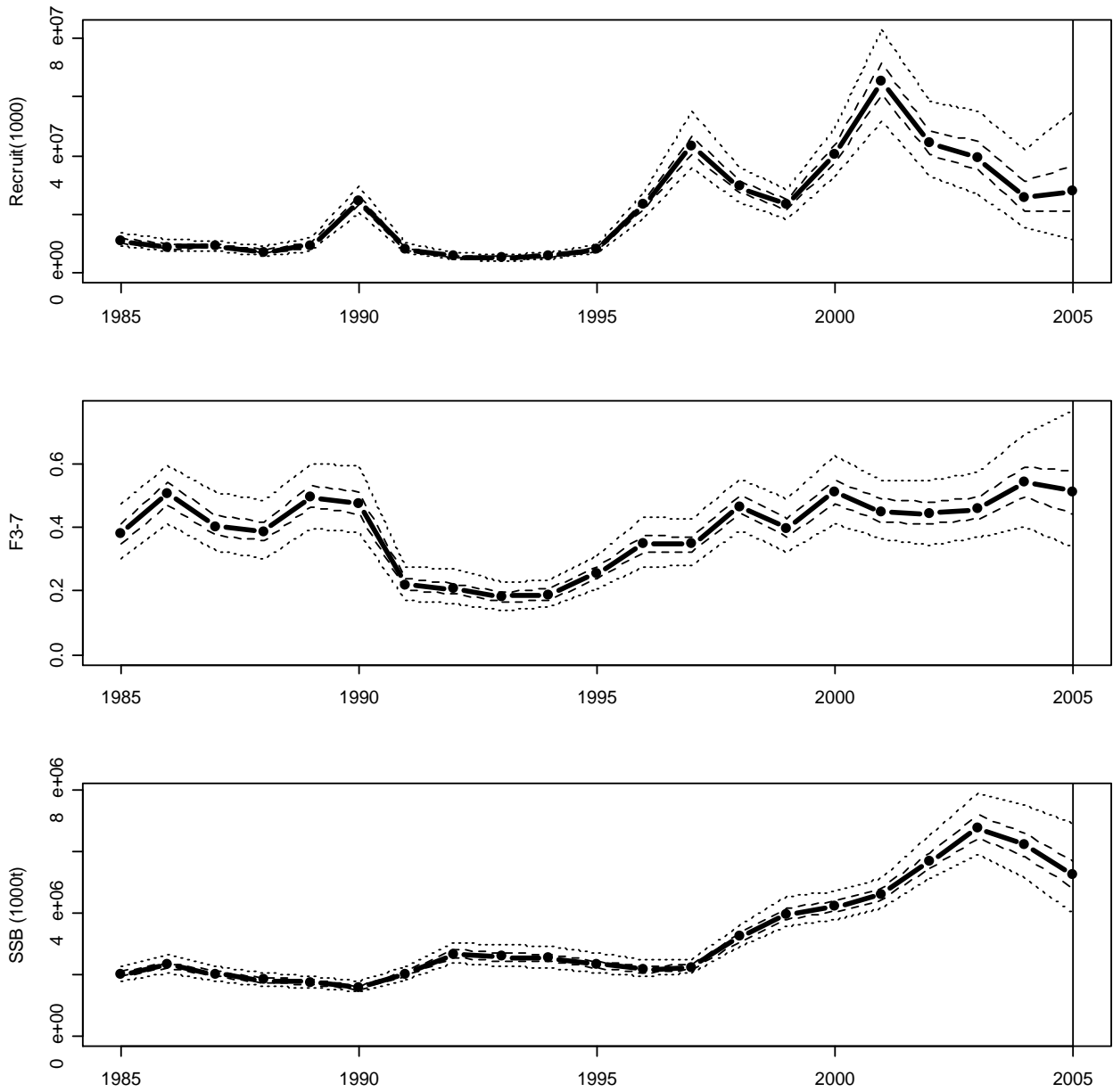
Figure 4.7.5.12 Blue Whiting, SMS. Posterior density (2.5, 25, 50, 75 and 97.5 percentiles) of average F and SSB estimated from 200000 Markov Chain Monte Carlo simulations.
