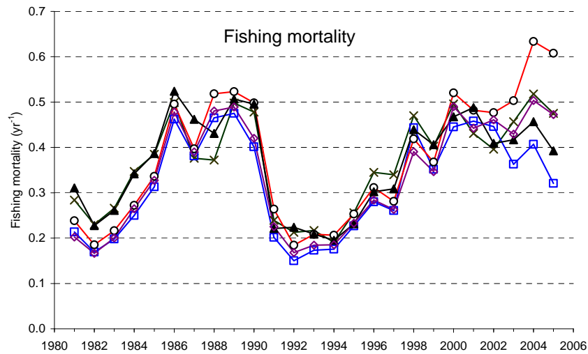
Figure 4.7.7.1. Blue Whiting: Comparisons between final AMCI, ISVPA, ICA, XSA and SMS assessments.
