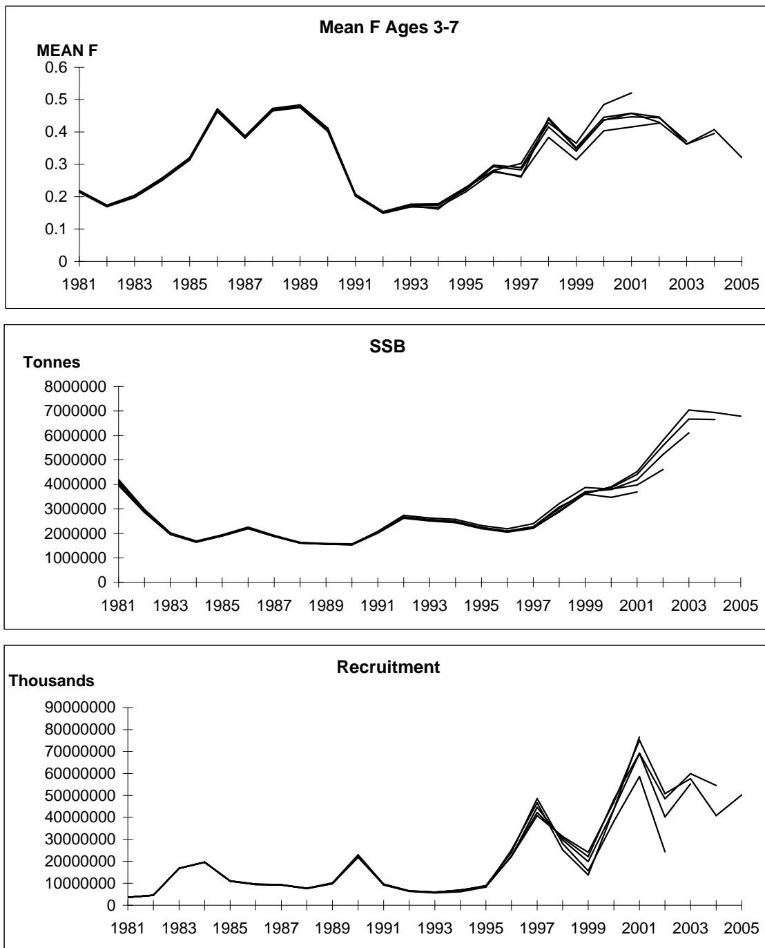
Figure 4.7.4.4. Retrospective ICA runs to 2001 using settings for final run 2006
