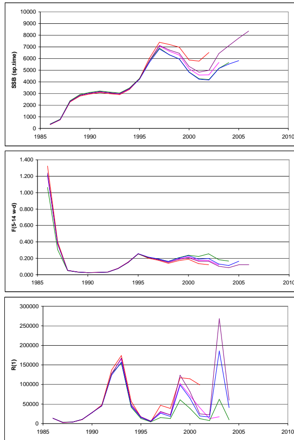
Figure 3.7.2.2.5. NSSH. Retrospective runs.
