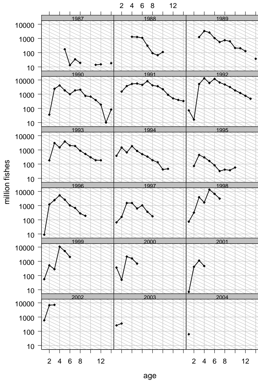
Figure 3.7.1.3. Norwegian spring spawning herring. Age disaggregated abundance indices from the acoustic surveys in the wintering areas in November-December plotted on log scale. The labels above each figure indicate yearclasses. The grey lines correspond to Z=0.4 .
