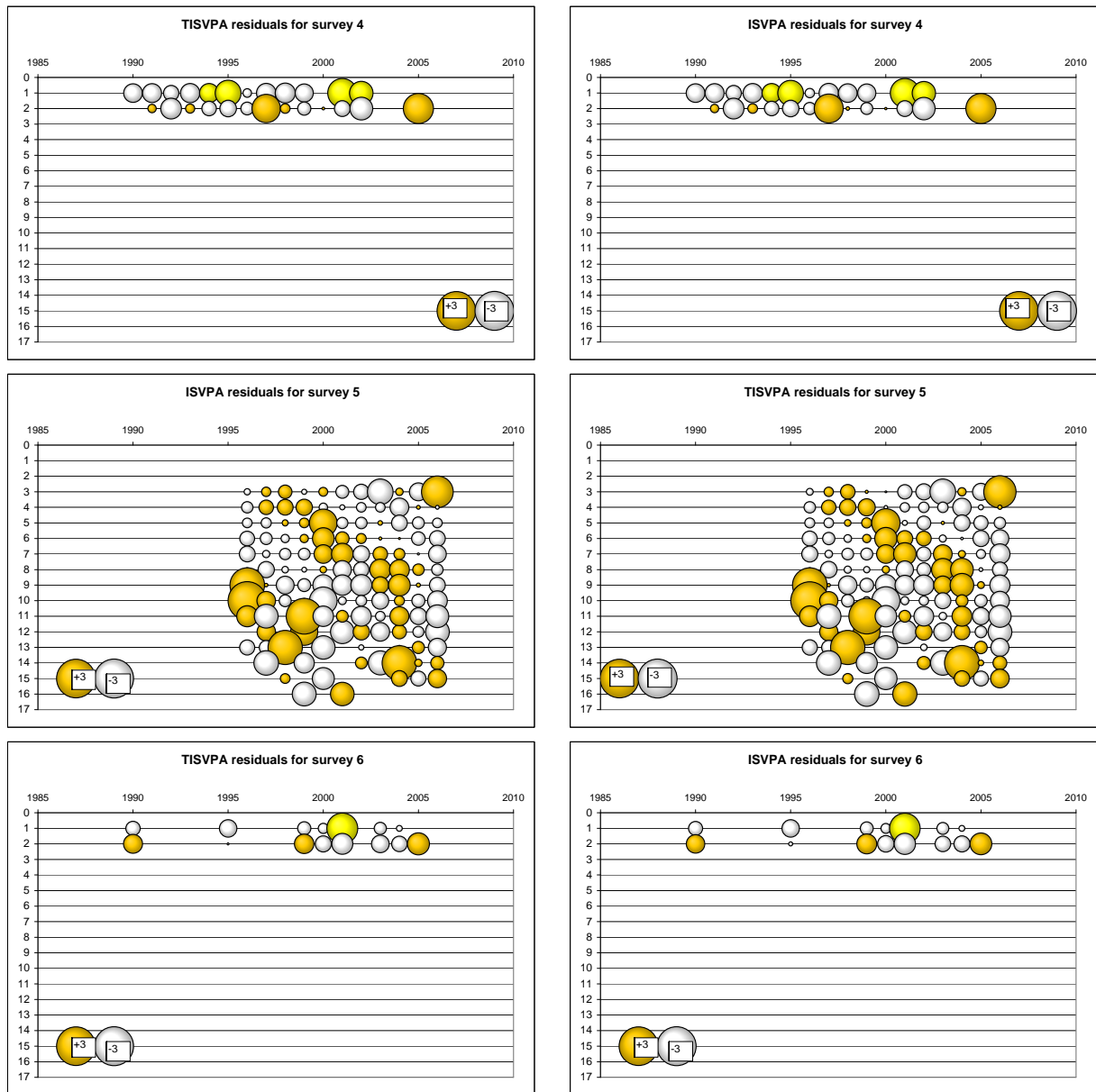
Figure 3.7.2.2.2 NSSH. Residuals in TISVPA and in ISVPA.
