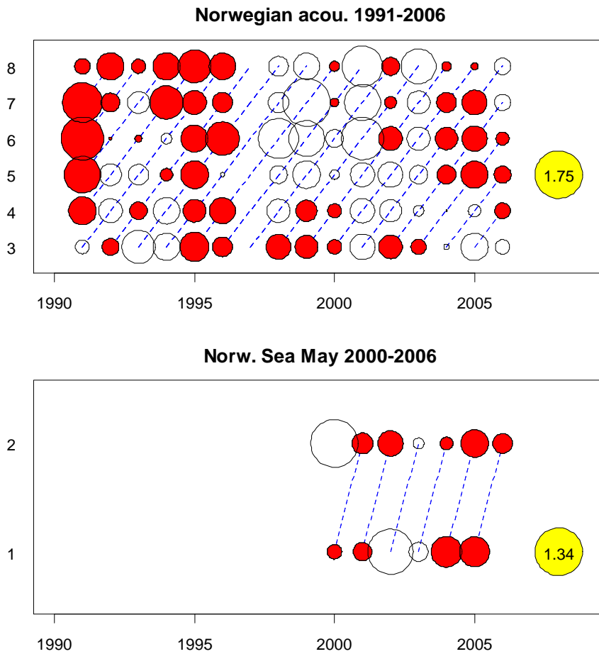
Figure 4.7.5.5 Blue Whiting, SMS exploratory run, residuals for survey observations. Red (dark) bubbles show that the observed value is bigger than the expected value.
