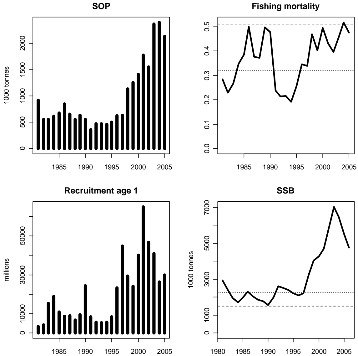
Figure 4.7.5.9 Blue Whiting, SMS. Stock summary, 1981-2005. (SSB in 2006 does not include age 1)
