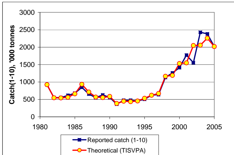
Figure 4.7.3.5. BW. Comparison of reported and TISVPA-derived theoretical catches
