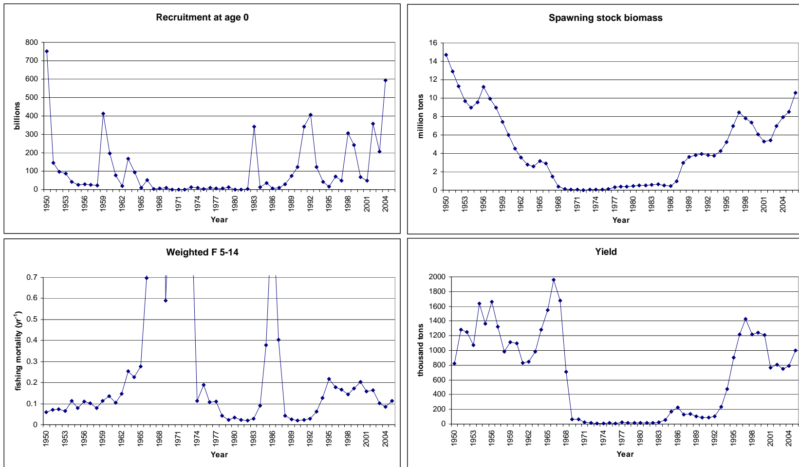
Figure 3.7.4.1. Norwegian spring spawning herring. Summary of final run.
