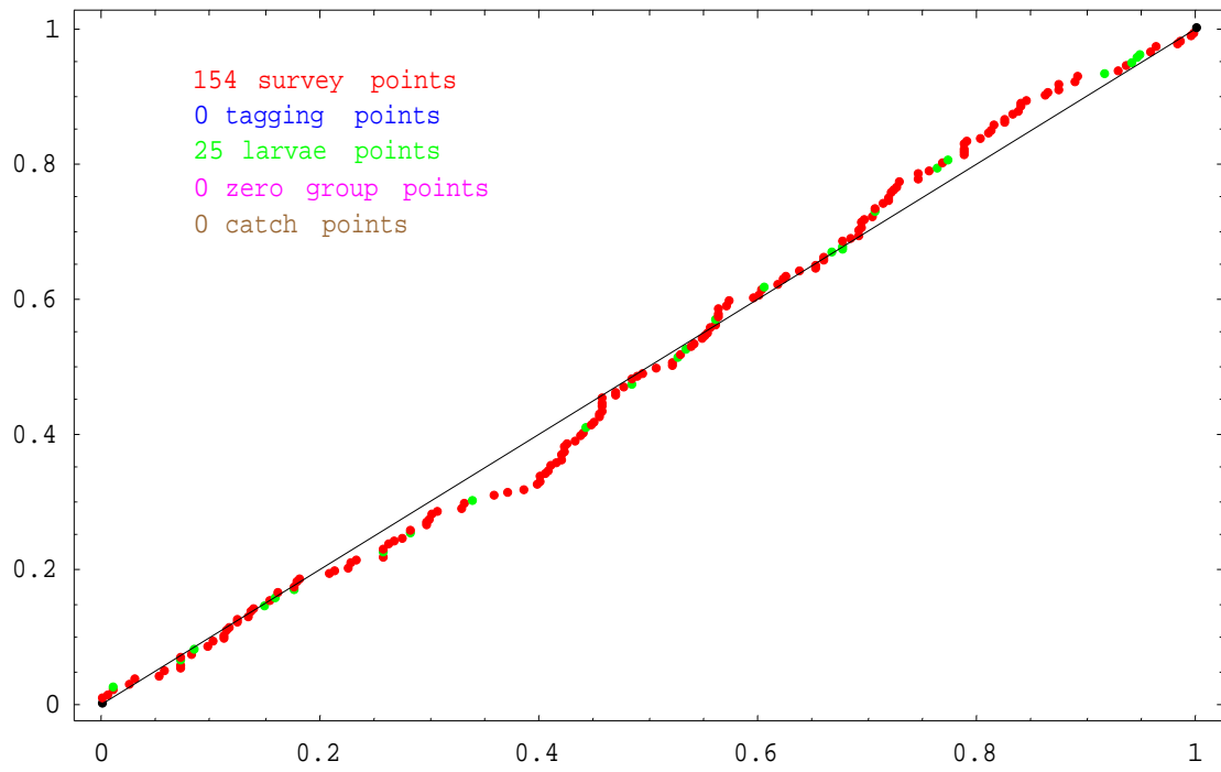
Figure 3.7.2.1.4. NSSH. Quantile-quantile plot the surveys on the adult stock and the larval data for the main SeaStar run.
