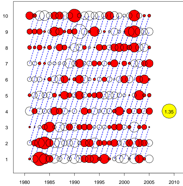
Figure 4.7.5.2 Blue Whiting, SMS. Catch residuals for run with bounds (25%) on CV of catch observations
